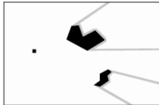
Figure 5: A 2D concealment computation. The black square is located at the viewpoint. The irregular polygons are objects in the environment.
