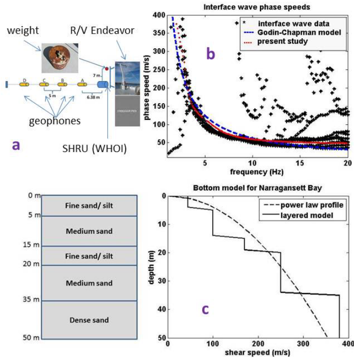
Figure 3: Phase velocity estimates (in black dots) from all possible geophone-event pairs (panel b). The experimental geometry for the Scholte wave data collection is shown in panel a. The continuous lines are theoretical group and phase velocity curves calculated using the Chapman-Godin approach (blue) and dynamic stiffness method (red). Panel c shows the shear wave speed profile (layered model for dynamic stiffness method and power law profile for Chapman- Godin model) used to calculate the theoretical group and phase speed curves. The layered sediment model is based on the sediment layers assumed (based on published data) for the location (shown to the left of panel c).
