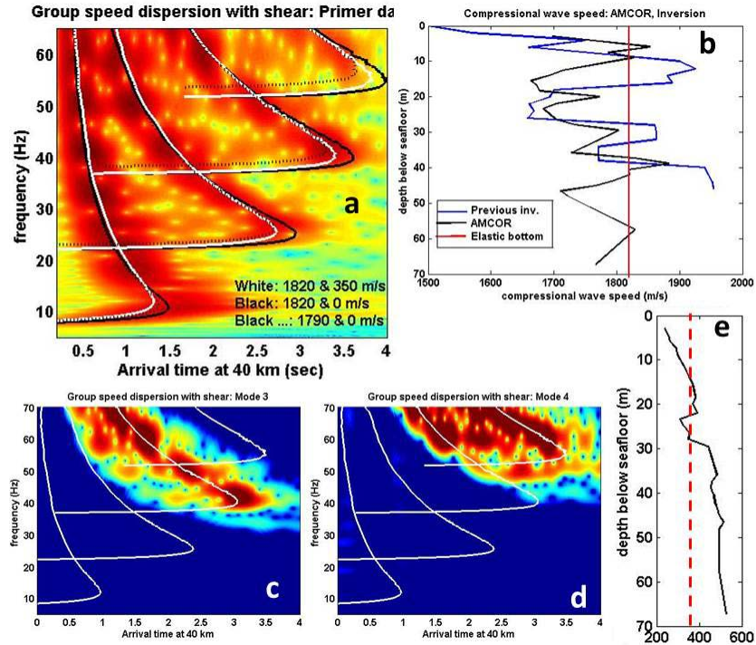
Figure 1: Panel (a) shows the calculated and observed modal arrival times. The continuous white lines are the modal arrival times calculated for a half space elastic sediment model with a compressional speed of 1820 m/s and a shear speed of 350 m/s. The broken black lines indicate that neglecting shear will have to be compensated by reducing the compressional wave speed to 1790 m/s. Panel (b) shows the compressional wave speeds in the sediment obtained by previous inversions and core data compared with the present estimate (1820 m/s). Panels (c) and (d) shows the theoretical group speeds (white lines) calculated using the half space model compared with mode 3 and mode 4 data. These time-frequency diagram were produced using the warping transform approach. Panel (e) compares the estimated shear speed (350 m/s) with shear speed computed using core data.
