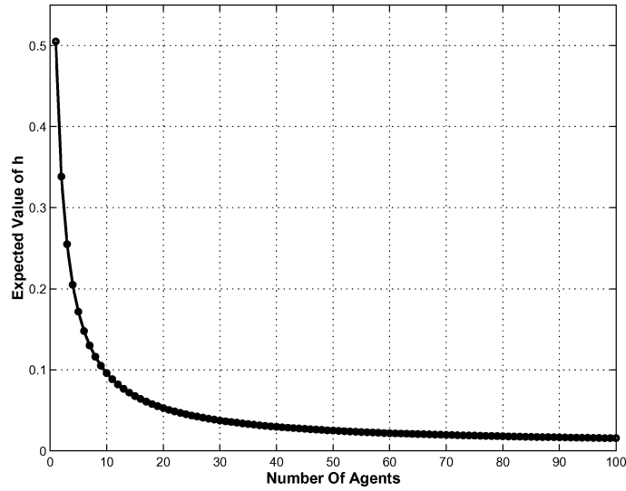
Fig. 7. The expected value of h (normalized), for the Single Agent Algorithm as a function of the number of agents.
