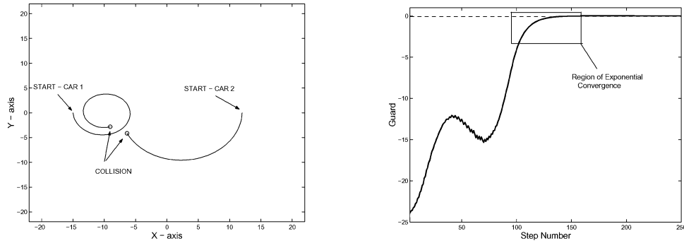
Fig. 3. The trajectory of the two robot vehicles in the plane is plotted (left); it is of interest to detect when they come within R feet of each other. The value of the event function (separation distance) as a function of step number is shown (right). The event function value converges to zero exponentially.
