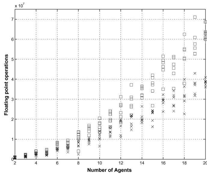
Fig. 10. Sample experimental results on the complexity of each algorithm as a function of the number of agents. Squares represent SAsim data and crosses are MASim data.
