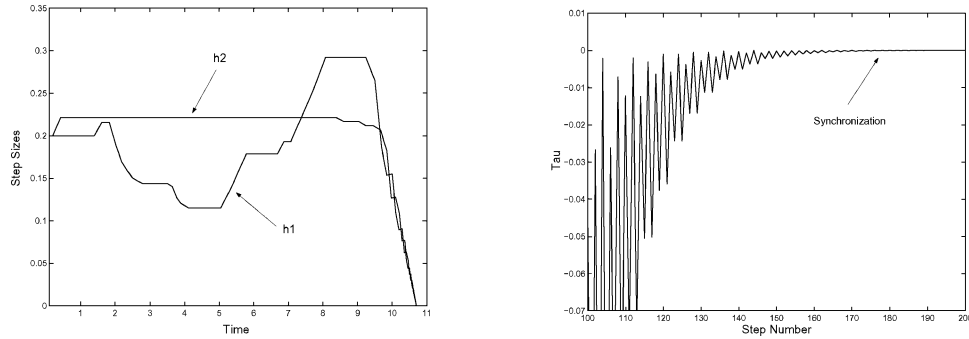
Fig. 4. Step sizes used in the first example are shown (left). h^1 and h^2 are selected independently away from the constraint but are brought into synchronization when an event is impending. The value of \tau (right), which is a measure of the discrepancy between the two local time clocks (i.e., asynchrony), rapidly decreases in magnitude as the event is approached.
