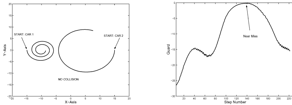
Fig. 5. The trajectory of the two robot vehicles in the plane for the second example (left). The initial condition is selected such that the two vehicles do not come within R feet of one another. However they do approach quite closely. The value of the event function as function of the step number is shown (right).
