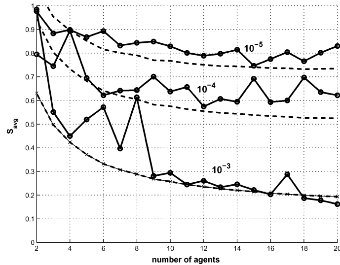
Fig. 11. Experimental results: Computational cost as a function of the number of agents, for various integration tolerances. Dash lines represent analytical predictions; while the solid line is the geometric mean of the experimental data.
