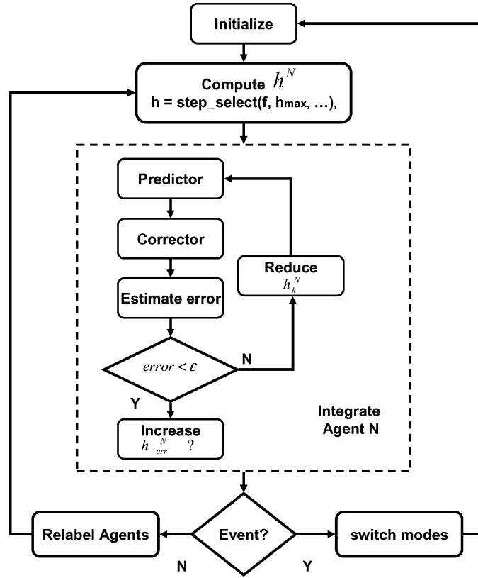
Fig. 1. The overall simulation algorithm MAsim presented in Section 5.
