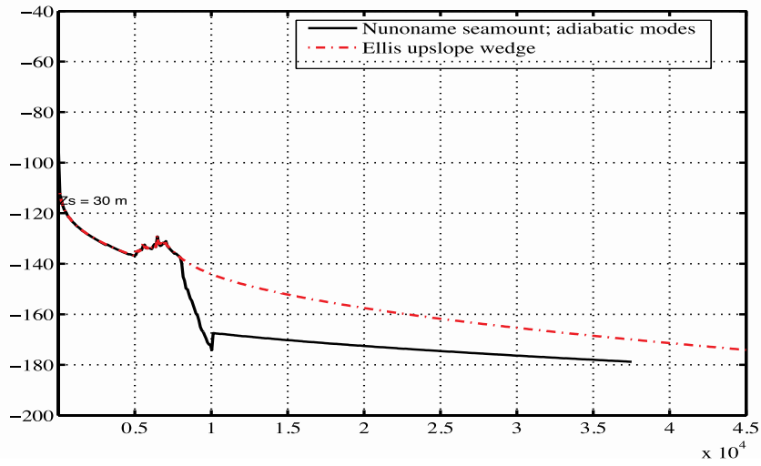
Fig. 1. A model-model comparison at 250 Hz of reverberation vs. time between Ellis' model and this model, for an offset ridge having a 2 deg. slope (modified Problem IV.1 from Zampoli et al.) using Lambert's rule and a winter profile and using a 1° beam and 50 m receiver
