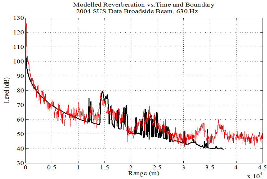
Fig. 2. Data model comparison for a SUS charge: reverberation vs. time at 630 Hz in the Malta Plateau, using Lambert's Rule (Coeff. = -37 dB) and the Boundary 2004 spring profile for a towed array broadside beam looking East (and West) going up the Ragusa Ridge. Originally the comparison was poor but wherever local slopes are greater than 1 degree the Lambert's coefficient was changed to -17 dB.
