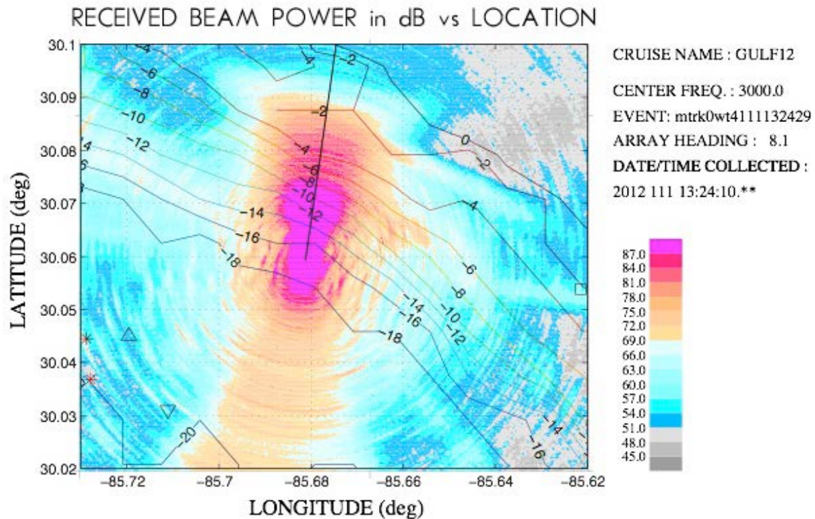
Fig. 3 Polar plot of reverberation vs. location using the FORA off Panama City, FL and a 0.1 s LFM from 2500–3500 Hz (triplet beamforming). Water depth 18 m; source depth 17 m; receiver depth 18 m. Symbols show the locations of shipwrecks and other man-made sources of clutter.
