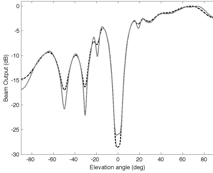
Figure 1: Beamformer output using data from 32-element array. The solid gray line uses the synthetic array approach with size 64 \times 64 CSDM and yields deeper nulls in the beamformer output compared to the dashed black line, which is the standard beamformer with CSDM of size 32 \times 32 .
