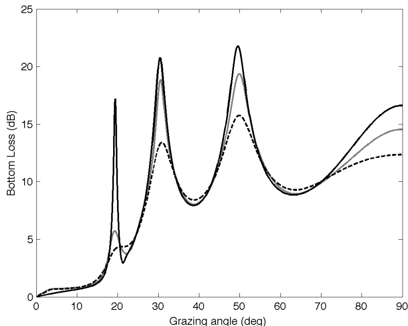
Figure 2: Black solid line is the true bottom loss; the dashed black line uses the standard beamforming with CSDM of size 32 \times 32 to estimate bottom loss from ambient noise. The gray line is the synthetic array that produces a CSDM with size 64 \times 64 to estimate bottom loss. The gray line is closer to the ground truth both from visual inspection and as measured by a mean-squared error estimate.
