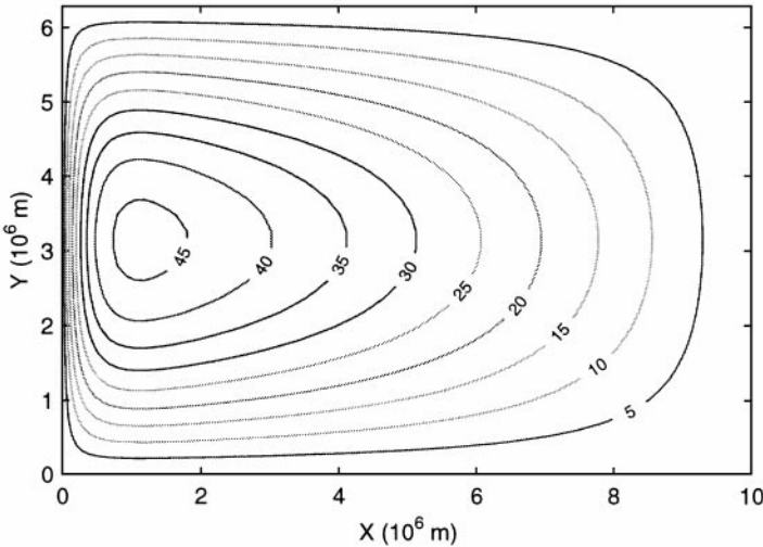
FIG. 2. Streamfunction ( \text{m}^2/\text{s} ) obtained from Stommel ocean model.
