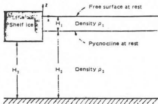
FIGURE 1. Diagrammatic representation of two-layer shelf-ice model (Clarke, 1978).
