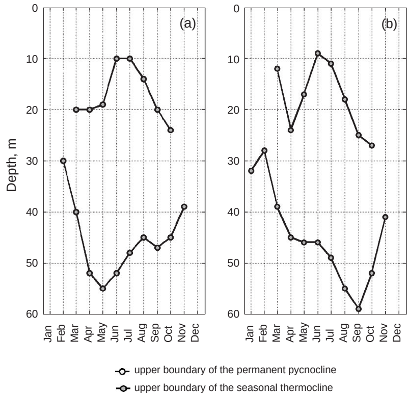
Fig. 8. Upper boundaries of the permanent pycnocline and seasonal thermocline in the (a) western and (b) eastern cyclonic gyres.
