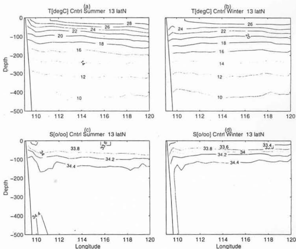
FIGURE 9. Thermohaline feature at the 13^\circ\text{N} zonal cross-section simulated by the control run: (a) summer temperature ( ^\circ\text{C} ); (b) winter temperature ( ^\circ\text{C} ); (c) summer salinity (psu), and (d) winter salinity (psu).
