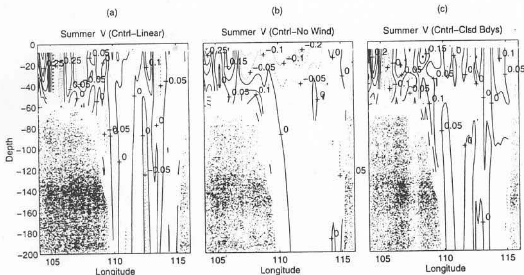
FIGURE 16. Summer latitudinal velocity anomaly ( \text{m/s} ) at the 6^\circ\text{N} cross-section, caused by effects of (a) nonlinearity, (b) winds, and (c) boundary forcing.
