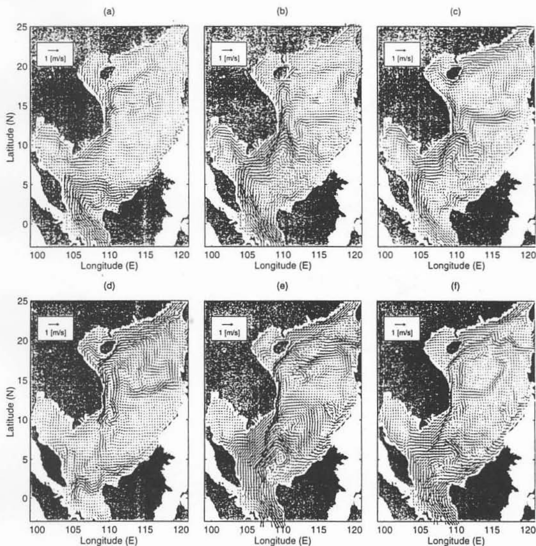
FIGURE 5. Surface circulation for control run on (a) May 15; (b) July 15; (c) September 15; (d) October 15; (e) December 15; and (f) March 15.
