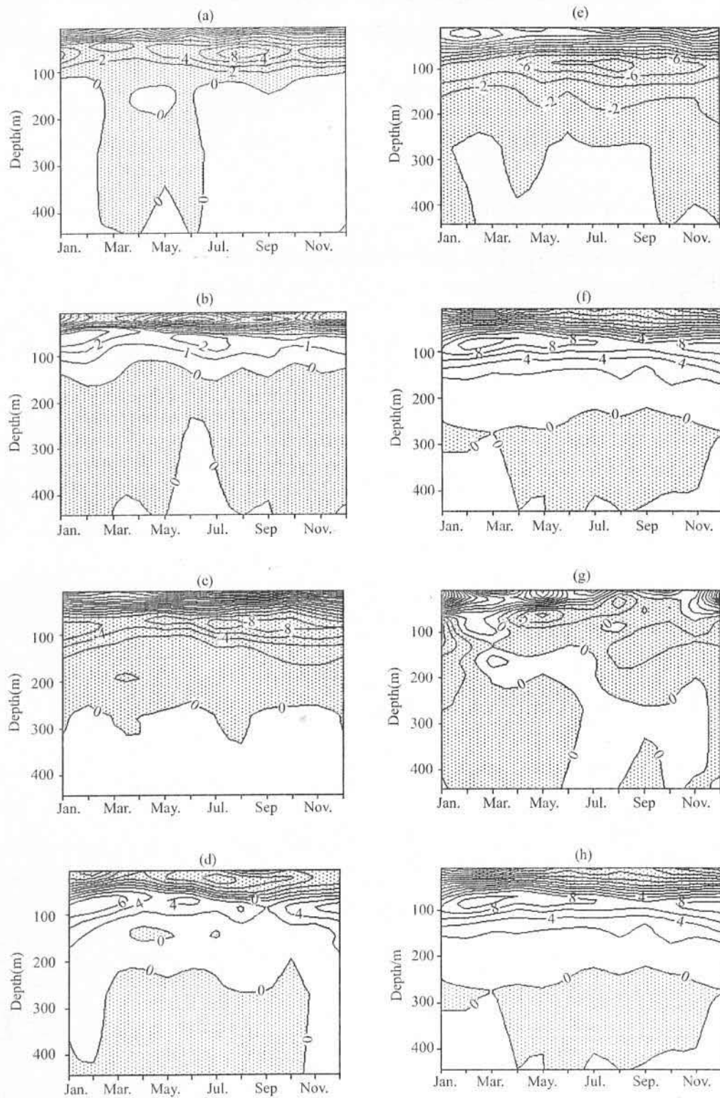
Fig. 5. Time-depth sections of meridional component of velocity(cm/s) along 1.352 3°N (left panels) and along 1.352 3°S (right panels)(Negative values are dotted). At 110°W(a,b), at 140°W (c,d), at 170°W (e,f) and at 165°E(g,h).
