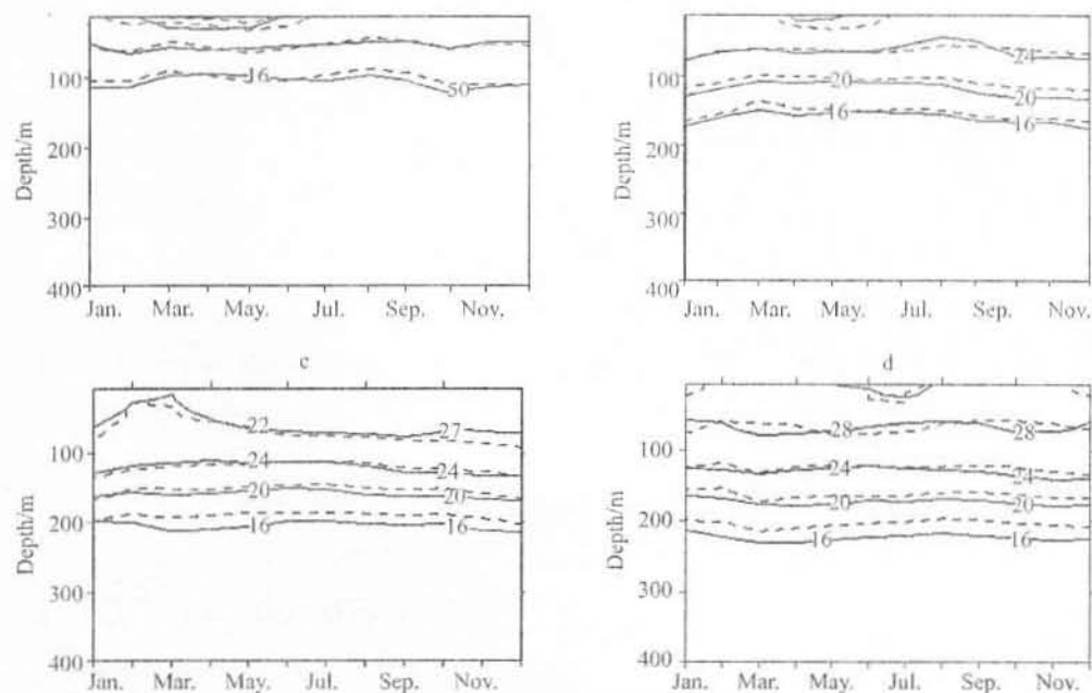
Fig. 3. Time-depth cross-sections of 14 averaged temperature ( ^{\circ}\text{C} ) along the equator observed from TOGA-TAO (dashed lines) and assimilated by SODA (solid lines) at 110^{\circ}\text{W} (a), at 140^{\circ}\text{W} (b), at 170^{\circ}\text{W} (c) and at 165^{\circ}\text{E} (d).
