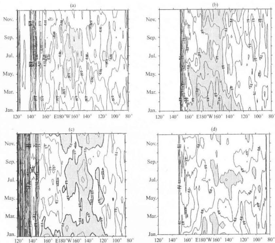
Fig. 4. Longitude - time section of equator-ward (a,b) northward(c) and southward(d) monthly mean transportation in the upper 300 m layer at 1.352^{\circ}\text{N} (c,a) and at 1.352^{\circ}\text{S} (b,d) ( values less than -0.5 are dotted (b,c).)
