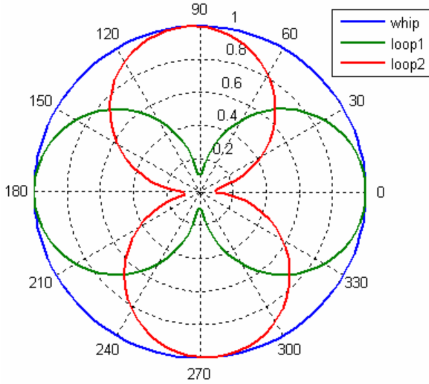
Figure 9 – Gain adjusted realistic antenna patterns.
