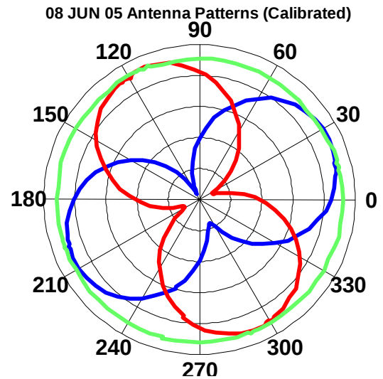
Figure 12 – After correcting the gains.
