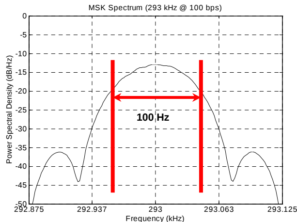
Figure 15 – Spectrum of an MSK signal.
