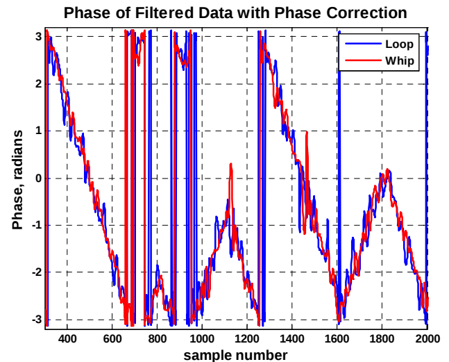
Figure 14 – Antenna outputs after phase adjustment.
