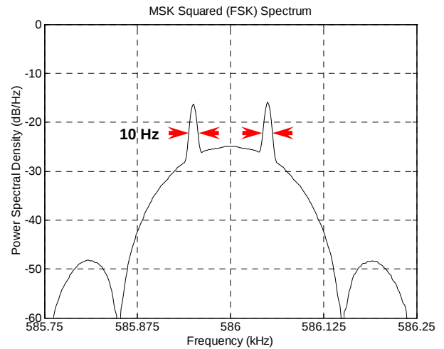
Figure 16 – Spectrum of a squared MSK or FSK signal.
