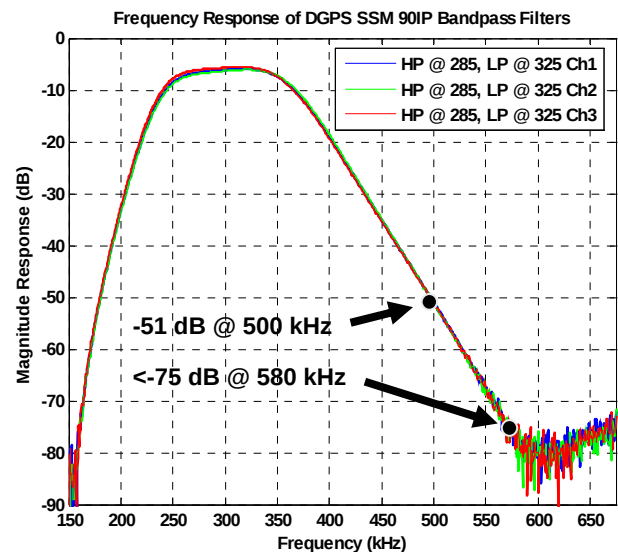
Figure 4 – Frequency responses (magnitudes) of the three anti-aliasing/bandpass filters.
