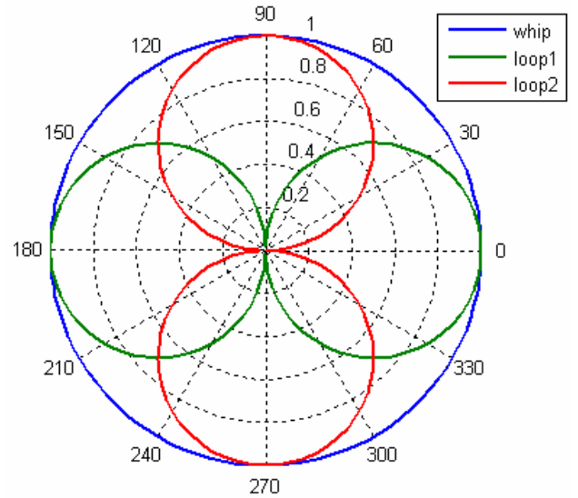
Figure 6 – Ideal antenna patterns.
