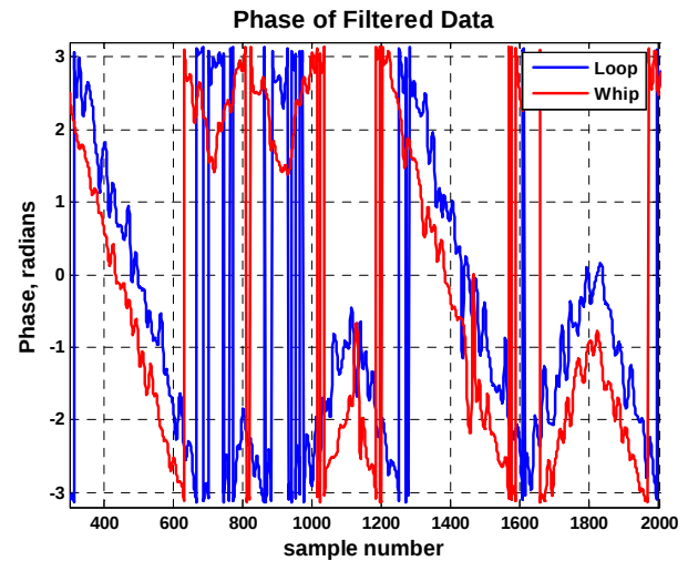
Figure 13 – Antenna outputs prior to phase adjustment.
