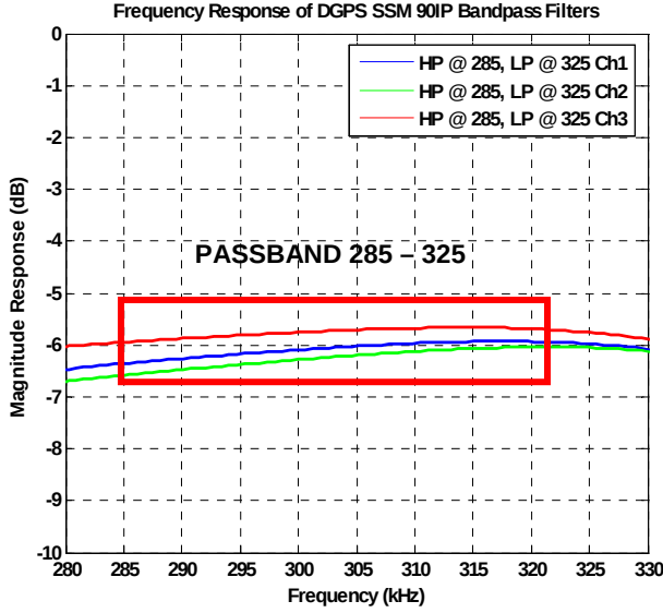
Figure 5 – Detailed look at the DGPS passband.
