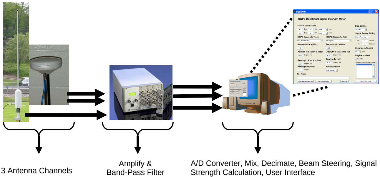
Figure 3 – System Diagram of Directional DGPS Signal Strength Receiver
