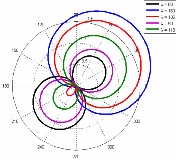
Figure 7 – Ideal steering to \phi=45^\circ with various angles to the null.
