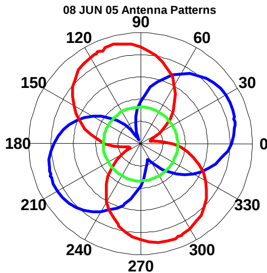
Figure 11 – Antenna patterns for our loops and whip.
