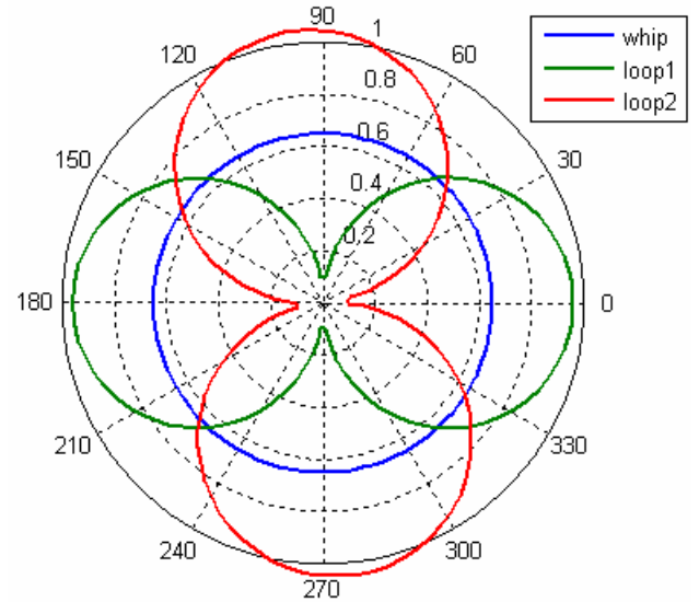
Figure 8 – Realistic antenna patterns.
