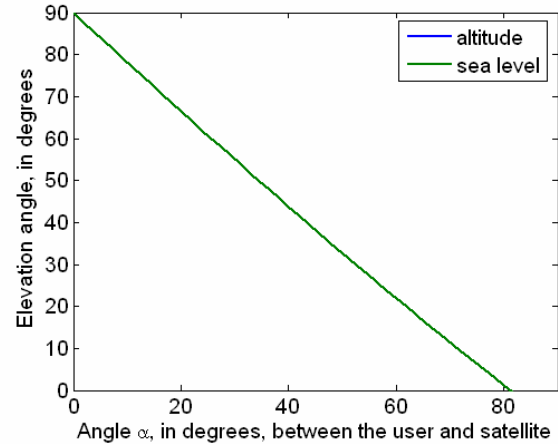
Figure 4 – Satellite elevation angle versus angle separating the user and satellite: user at sea level and user at 4.4 km altitude.
