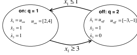
Figure 4: The system dynamics of the thermostat.
