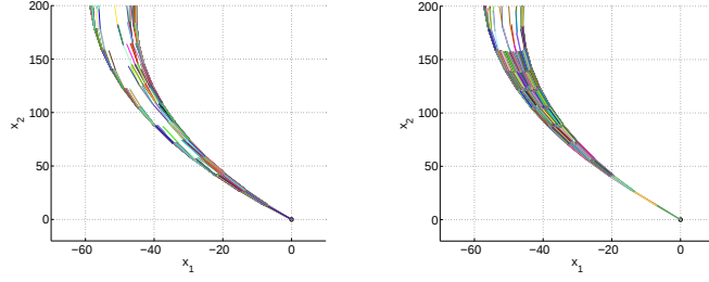
Figure 7: RRT for a linear system using the Euclidean metric ( left ) vs. a History-based selection of proximal node ( right ). After 5000 nodes the explored region of the reachable space is much more densely covered when using the weighting.
