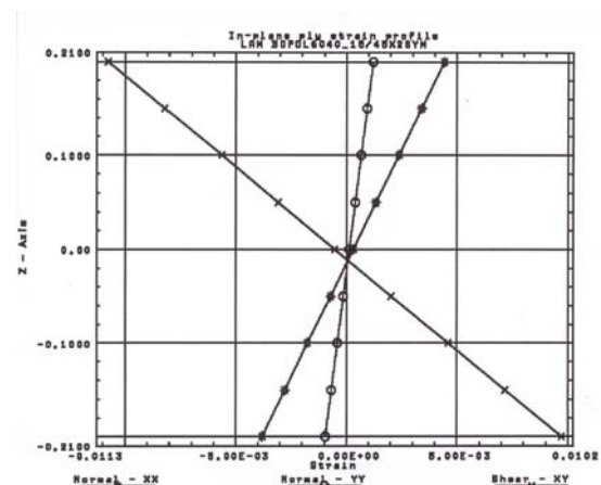
Figure 6: Strain distribution for symmetric laminate
