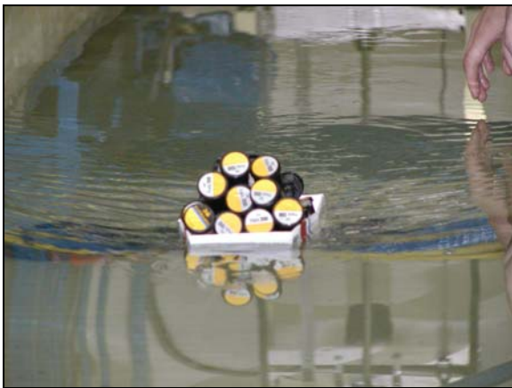
Figure 3: Balsa model in tank
