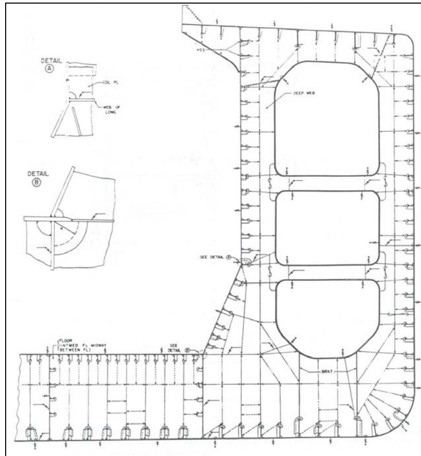
Figure 5: Midship Construction Section 2
