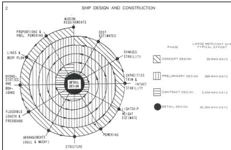
Figure 1: Naval architecture design spiral 2
