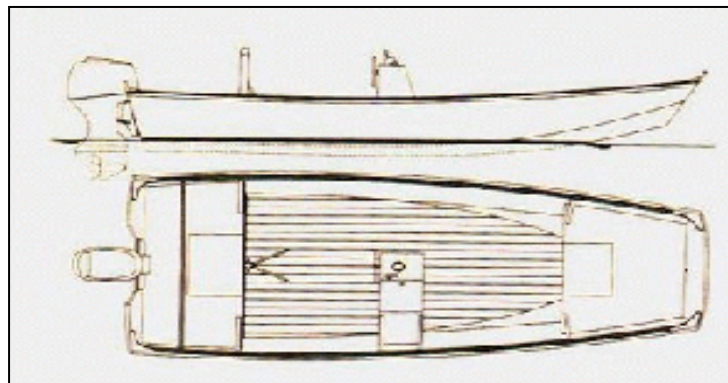
Figure 6. Eighteen foot garvey design used for composite group project.
