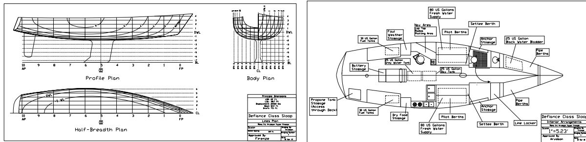
Figures 7-10: Capstone design course project submissions, including sail plan, tank test photo, lines plan, and accommodations plan.
