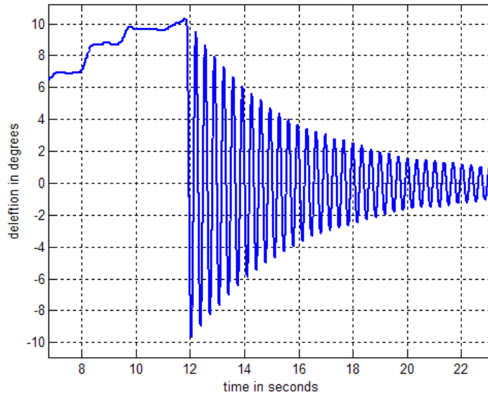
Figure 6: Impulse Response of Robotic Link
