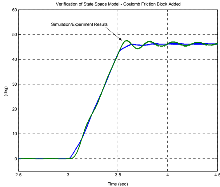
Figure 15: Simulation and Experimental Results with Friction Block
