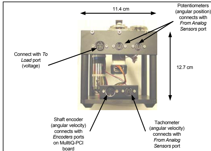
Figure 3: Quanser DC Motor
