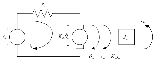
Figure 7: DC Motor Representation
