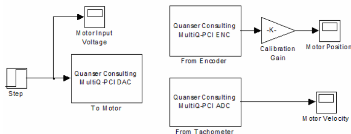
Figure 5: SIMULINK Diagram for DC Motor Experiment
