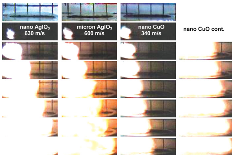
Figure 4 Video images of the combustion of three thermite samples in air. The images at the top show the samples prior to combustion, with a 45-mg line of powder placed on an aluminum support. A grid directly behind the sample has a spacing of 10.8 mm between lines. Samples were ignited by a spark from a wire attached to a tesla coil (tip of wire visible in the upper left corner of the top images). Images were recorded at 10- \mu s intervals, using a 2- \mu s exposure. The Al in this study is 80 nm from NanoTechnologies. The CuO in this study is 45 nm from Technanogy. Each sample was fuel rich in this study with equivalency ratios of 1.12 for the nano AgIO 3 material, 1.06 for the micron AgIO 3 material, and 1.27 for the CuO material.
