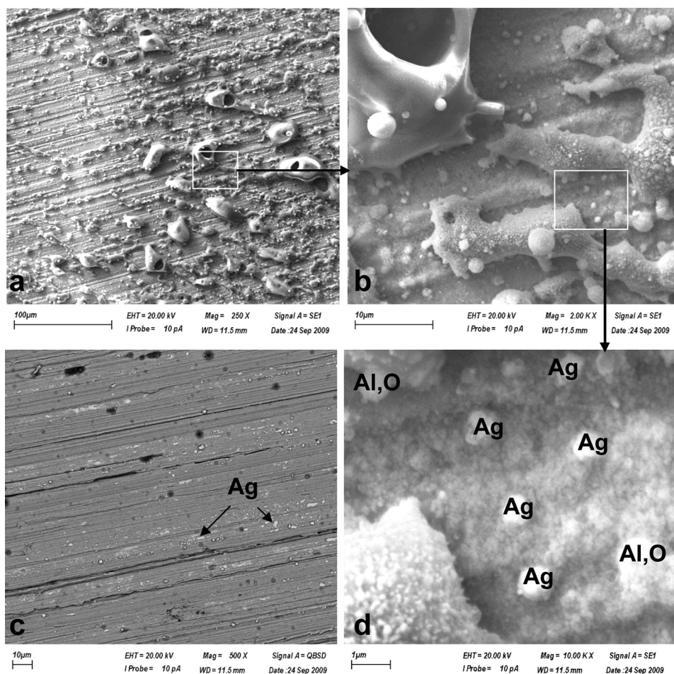
Figure 8 Scanning electron micrographs of reaction products from spark initiated nano Al/AgIO 3 (20 mg) deposited on a copper plate. Micrographs a, b, and d (taken at different magnifications) show the region of the copper plate that was positioned 10 mm directly above the sample. Micrograph c shows a region of the copper plate that was 10 mm distant from the spot of the top micrograph. Micrograph c was taken in the quantum backscatter mode, where the light elements (Al, O) appear as dark spots in the image, while the heavy elements (Ag, I) appear as light spots. Small islands of elemental Ag (essentially free of iodine) are marked in micrograph c. The nearly horizontal lines result from abrasive polishing of the copper plate. The Al was from Nanotechnologies, and the AgIO 3 was synthesized (181 nm).
