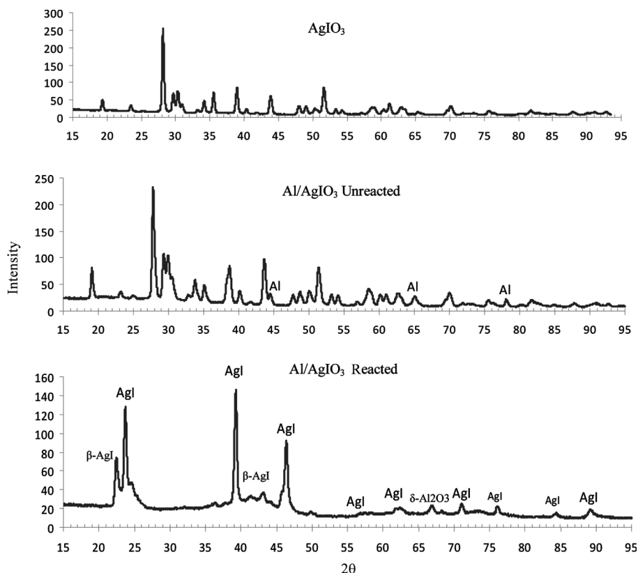
Figure 7 XRD patterns (Intensity vs. 2\theta ) for pure \text{AgIO}_3 , along with the thermite before and after reaction in the pressure cell. The major detectable reaction product is \text{AgI} . Unless otherwise noted, the \text{AgI} peaks are \gamma\text{-AgI} . The thermite was \text{Al} (ALEX) and synthesized \text{AgIO}_3 (156 nm) with an equivalence ratio of 1.0.
