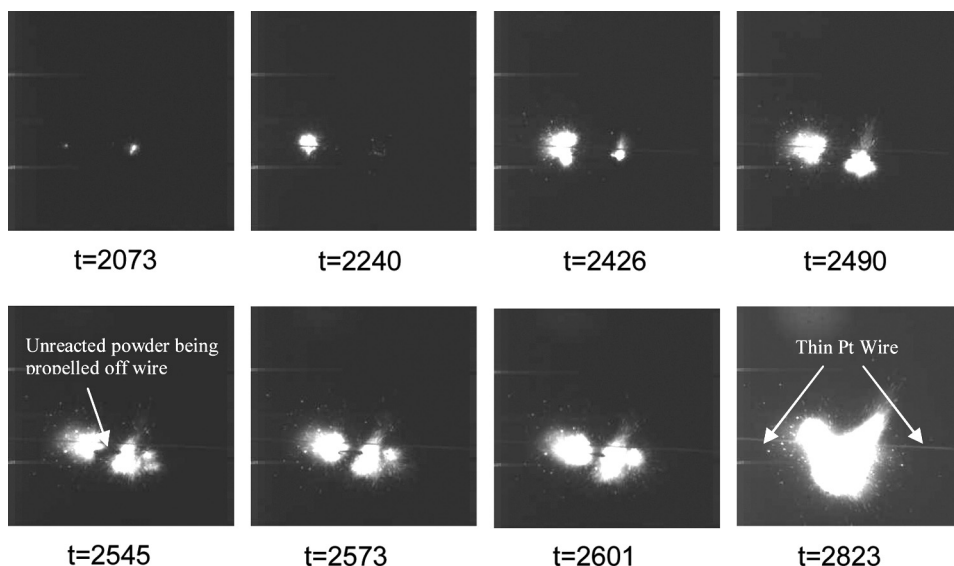
Figure 3 Sequential snapshots of Al/AgIO 3 burning in air. The wire can only faintly be seen, and remains stationary throughout the burning. The thermite is Al (ALEX) and AgIO 3 (156 nm), with an equivalence ratio of 1.0.
