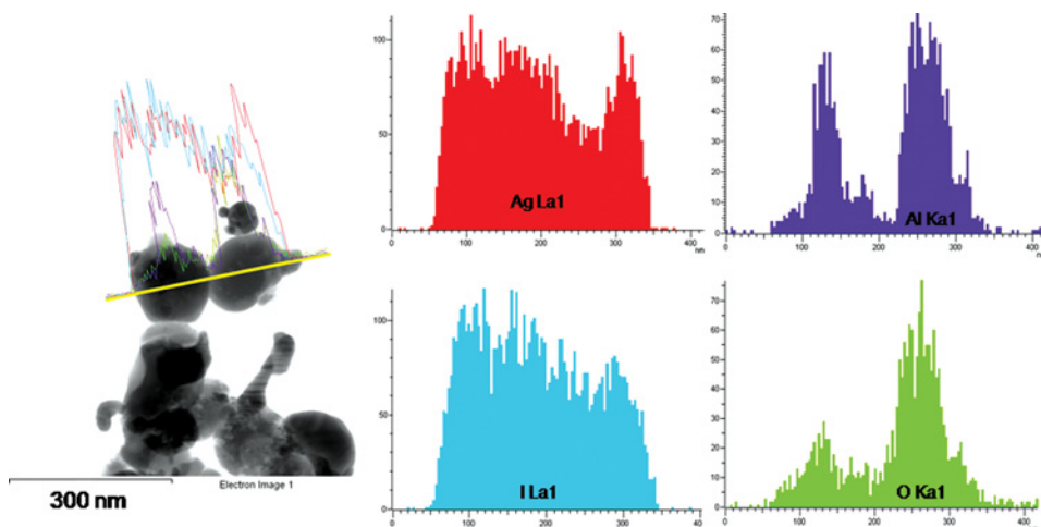
Figure 6 TEM image and 1D elemental linescan (using EDS) across two adjacent particles of Al/ \text{AgIO}_3 reacted in the pressure cell. Note the presence of an Al/O core surrounded by AgI in each particle. The extra (green) line shown in the image was carbon from the film. The thermite was Al (ALEX) and synthesized \text{AgIO}_3 (156 nm) with an equivalence ratio of 1.0.
