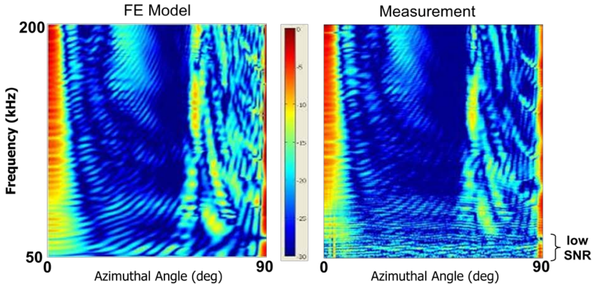
Figure 25. Validation of COMSOL-based FE solution for scattering by a free-field 5:1 solid Al cylinder.
