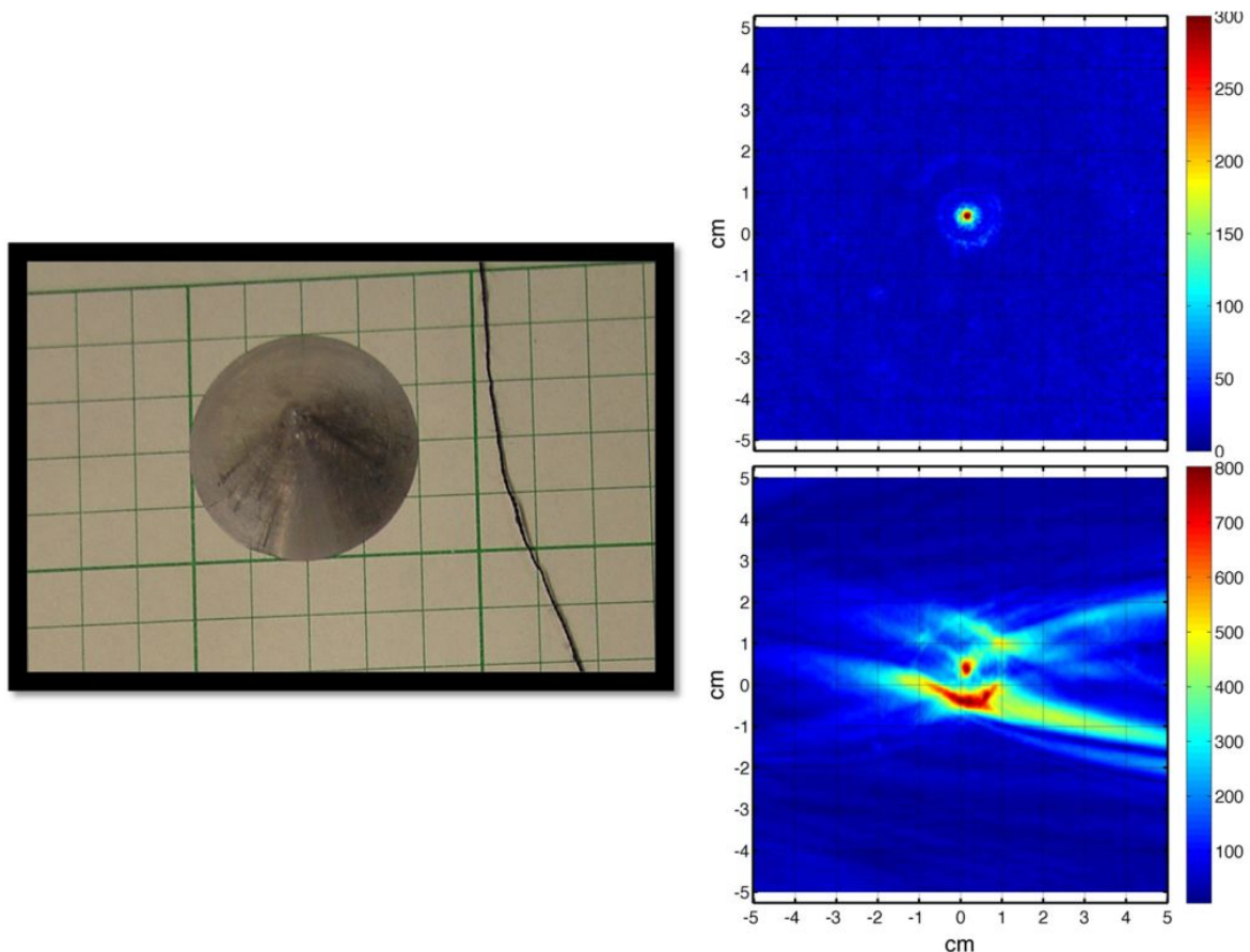
Figure 17. Picture (left) of .8 inch solid Al cone resting on graphing paper with 1 inch large squares (the small squares are .2 inch). Monostatic CSAS image of the cone resting proud on simulated sediment (upper right). Bistatic CSAS image of the cone resting proud on simulated sediment (lower right). The data are plotted on a linear scale and the amplitudes have not been corrected to account for the different sensitivities of each receiver. As a result, the absolute amplitudes are not comparable between the two images.
