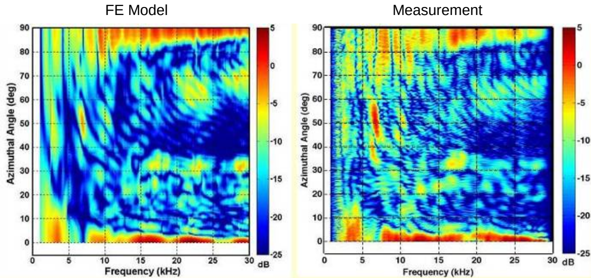
Figure 26. FE vs measurement comparison for scattering by a 5:1 solid Al cylinder deployed proud on the sand bottom of the NSW PCD freshwater pond.
