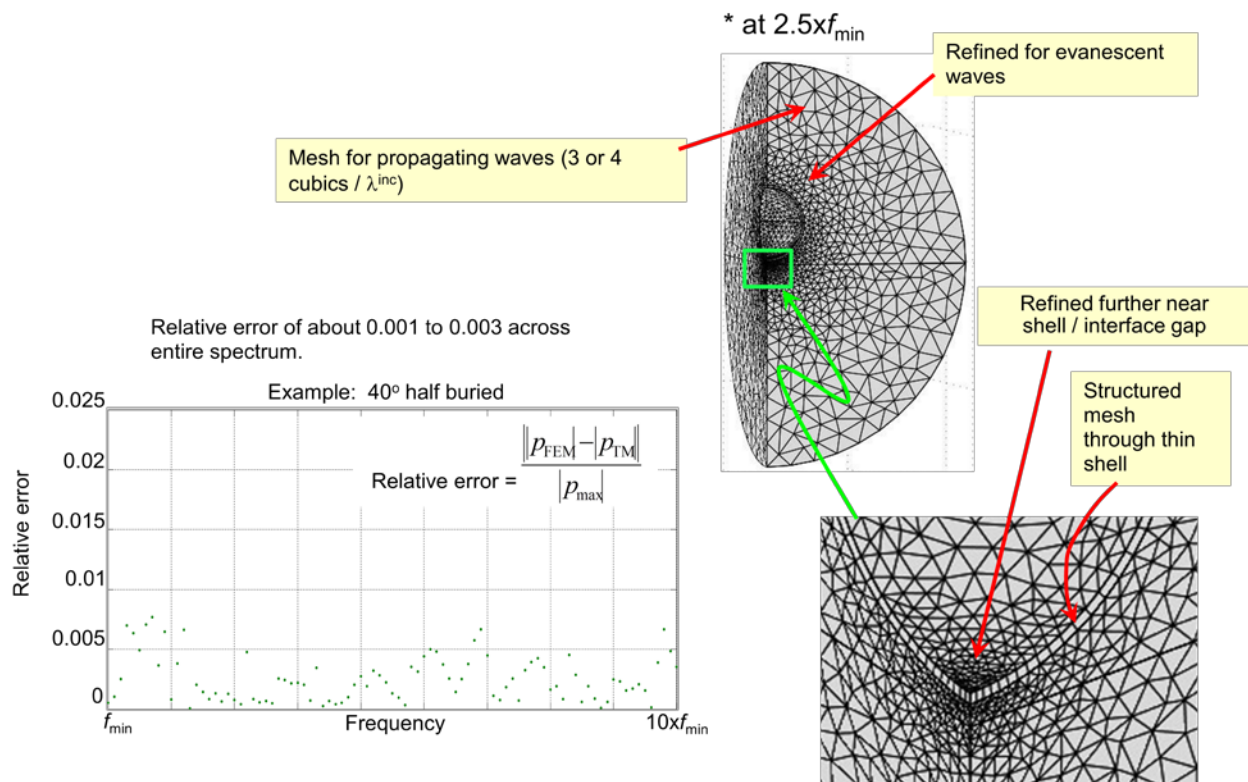
Figure 23. Mesh refinements formulated for scattering by a proud spherical shell.
