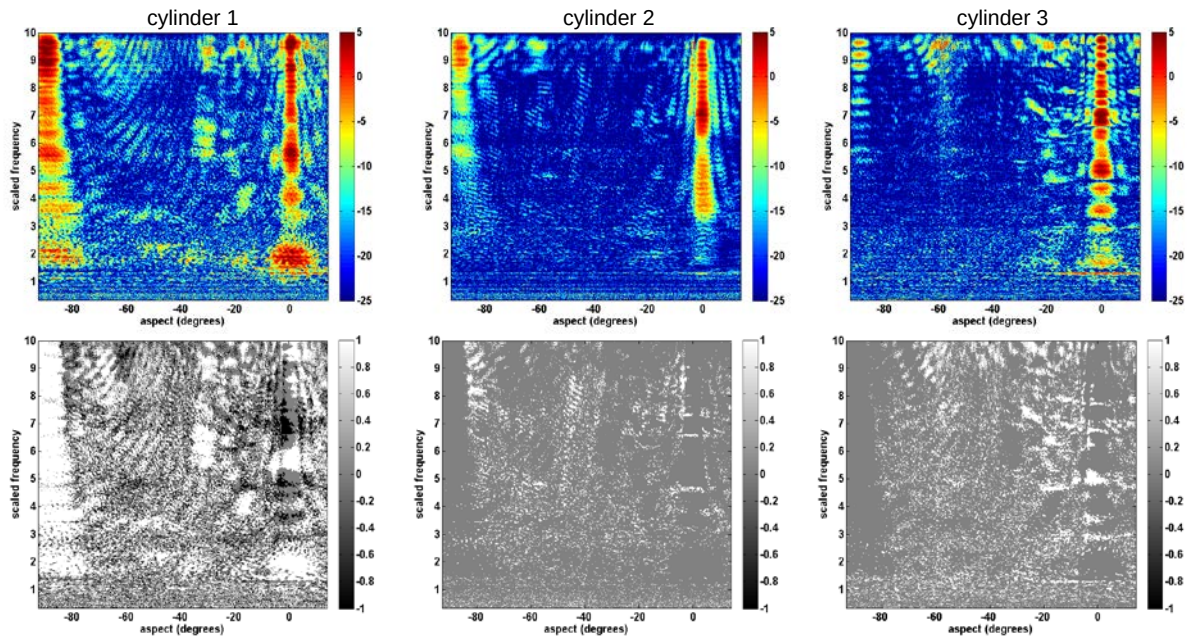
Figure 33. Among a set of 3 like- shaped cylinders, a feature selection tool is applied to look for phenomena in the acoustic color of each target (top row) that is unique to that target (white or black regions in the corresponding plot below).
