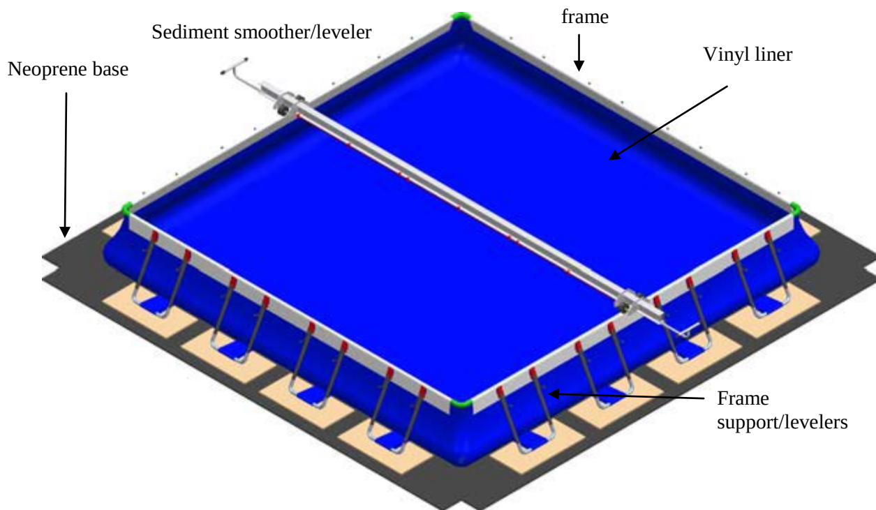
Figure 40. Pictorial of the sediment tank designed for high-grazing-angle data collection from bottom targets.
