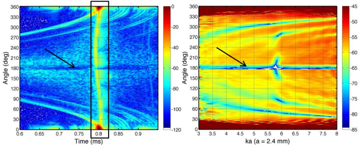
Figure 21. Time-domain bistatic scattering data (left) for a proud 2.4 mm solid stainless steel sphere plotted on a dB scale normalized to the brightest pixel. Bistatic target strength (right) from a windowed subset (black rectangle) of the time-domain data isolating the target scattering. The horizontal null (black arrows) in both plots is caused by the source blocking the receiver at 180° (backscattering), see Fig. 7 at \phi = 0^\circ .
