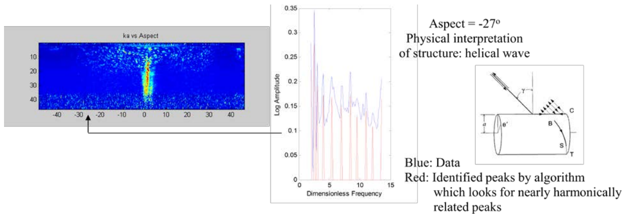
Figure 34. Excitation of surface Rayleigh waves at -27^\circ target aspect on a solid Al cylinder produces quasi-periodic structure in its target strength plot.
