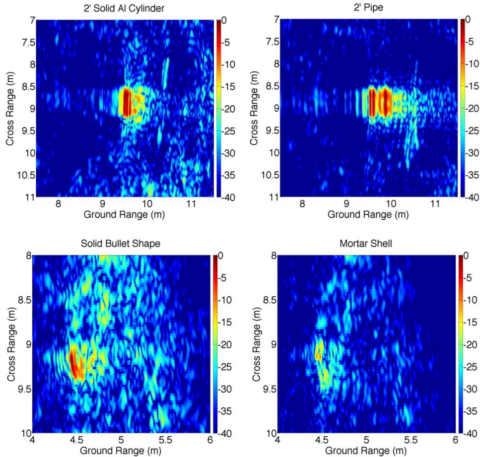
Figure 9. Backscatter SAS imagery processed from data collected around target broadside at 20^\circ (top images) and 40^\circ grazing angles (bottom images).
