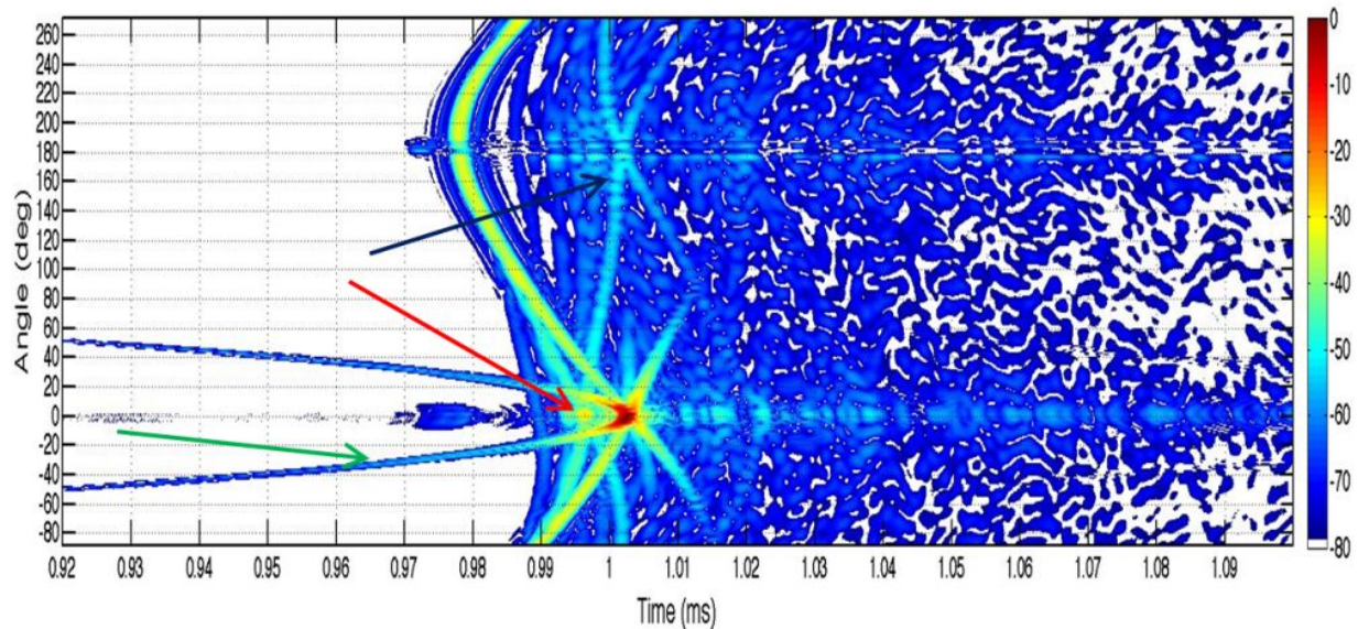
Figure 18. Bistatic time-series data for a free-field 1 inch diameter solid stainless steel sphere. The source and receiver configuration is shown in Fig. 7 but the angle origin is shifted by 180^\circ from \varphi . The time-domain data are plotted on a dB scale normalized to the brightest pixel. Backscattering is at an angle of 180 degrees and forward scattering is at 0 degrees. The arc (green arrow) corresponding to sound that travels directly from the source to the receiver has a bright enhancement at 0 degrees when the source and receiver are perfectly aligned. Two elastic responses related to surface waves are indicated by the black and red arrows.
