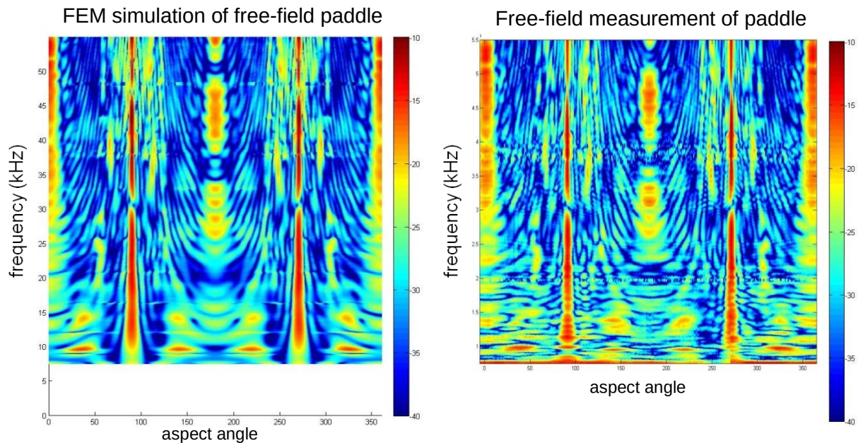
Figure 27. Comparison of FE simulated and measured free-field target strength plots for WSU's "paddle."
