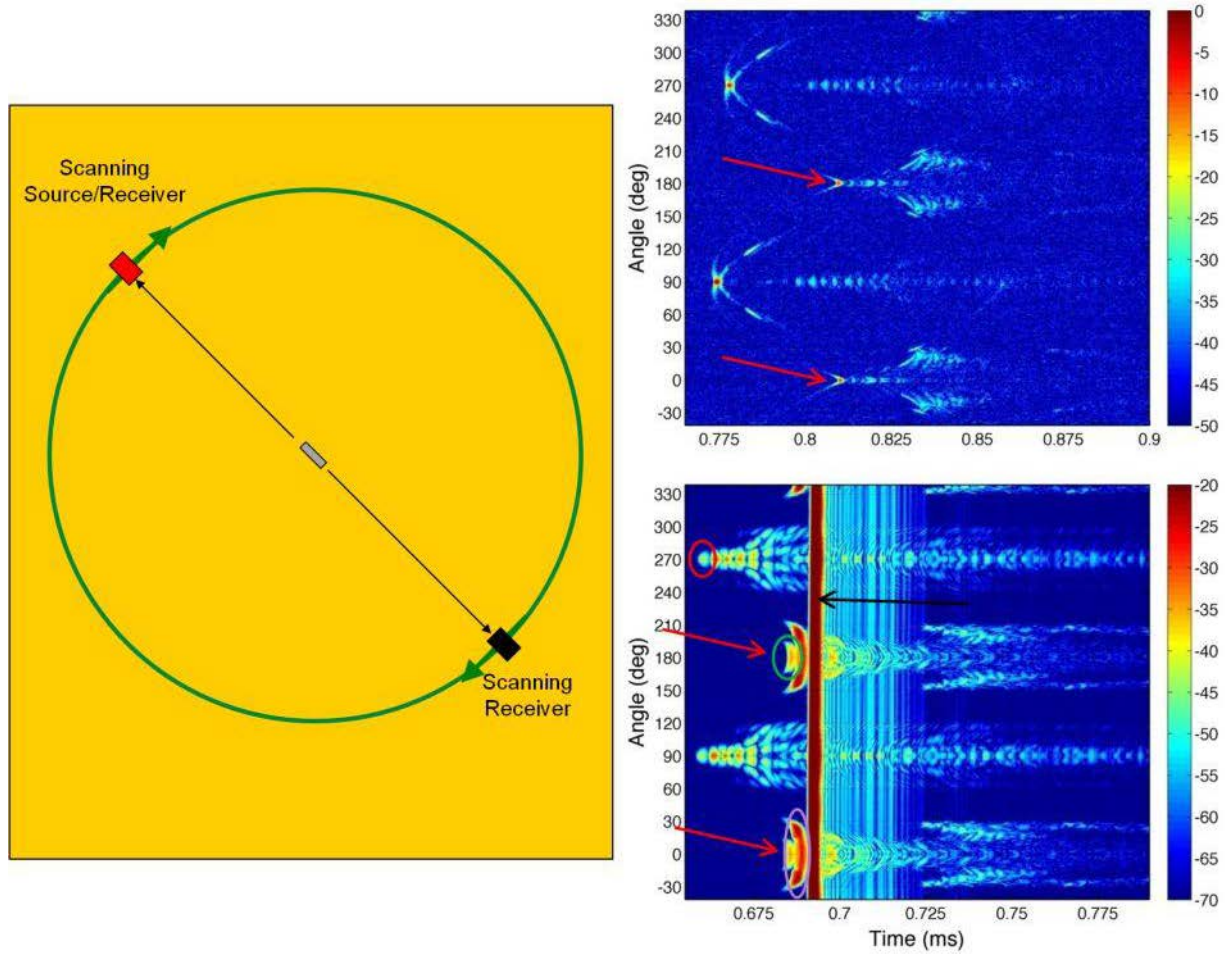
Figure 19. Diagram (left) of the circular-scan setup for free-field target measurements having a monostatic source/receiver with a bistatic receiver mounted directly across the circular scan line. Both the source/receiver and the bistatic receiver are translated on a circular path simultaneously, while keeping their relative positions fixed. The bright vertical lines (black arrow) are not target related. They are the result of sound traveling directly from the source to the receiver. A stationary 5:1 .5 inch diameter solid aluminum cylinder is suspended in the center of rotation. The backscattering time-series data (upper right) and the forward scattering time-series data (lower right) are plotted as a function of aspect angle. The time-domain data are plotted with a 50 dB dynamic range and normalized to the brightest pixel in each plot. At angles of 0 and 180 degrees (red arrows) the source is broadside to the target.
