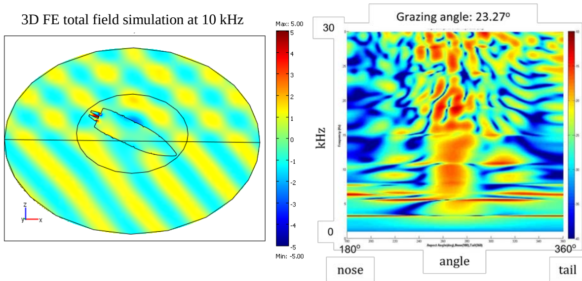
Figure 29. 3D FE simulation of scattering by artillery shell embedded in a sand bottom with a 25^\circ tilt. Plots of total field (left) and backscatter target strength vs. frequency and aspect angle (right) are shown for a plane wave incident at a 23.27^\circ grazing angle.
