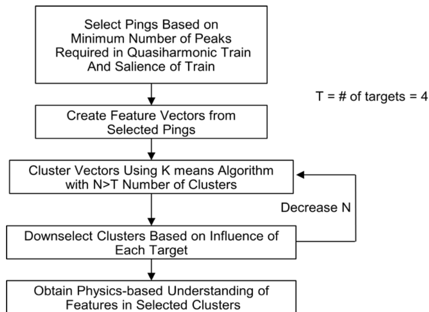
Figure 35. Process for using elastic information in sonar data to discriminate between 4 cylindrical targets with the same size and shape.
