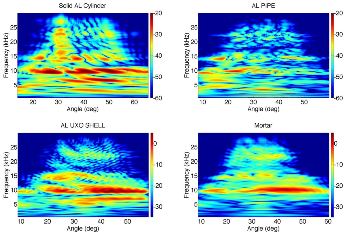
Figure 10. Backscatter acoustic color processed from data collected around target broadside at 20^\circ (top plots) and 40^\circ grazing angles (bottom plots).
