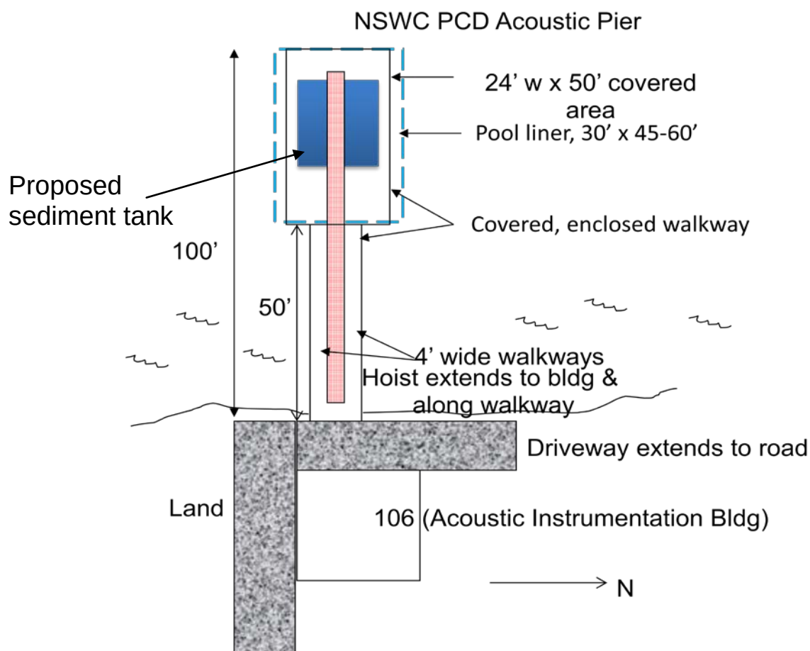
Figure 39. Schematic of the NSW PCD Acoustic Pier Facility including the sediment tank (blue) to be deployed at the bottom of the lined freshwater pool. Sonar hardware suspended from the rotator moved along the overhead rail (red) would be able to detect targets in the tank at high grazing angles.
