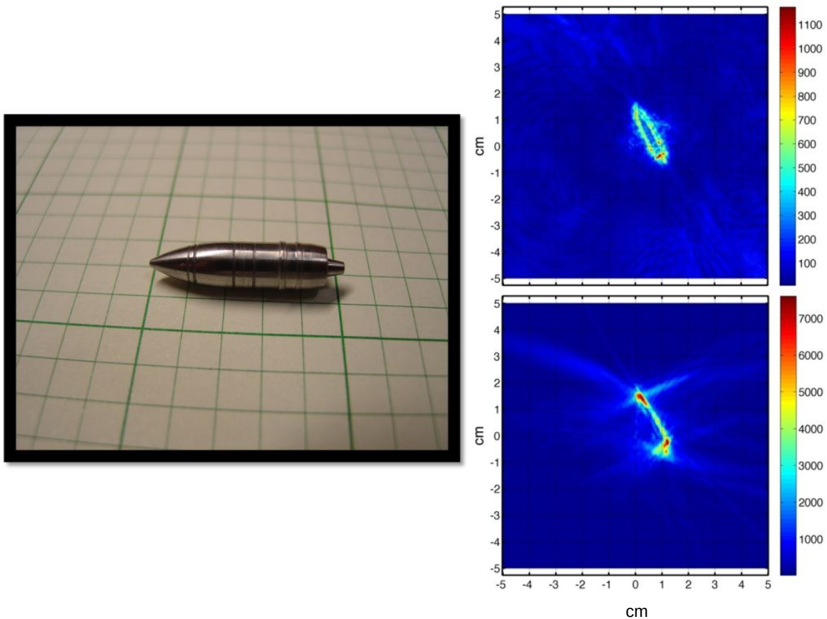
Figure 16. Picture (left) of 1/16 scale solid Al UXO replica resting on graphing paper with 1 inch large squares (the small squares are .2 inch). Monostatic CSAS image of the UXO resting proud on simulated sediment (upper right). Bistatic CSAS image of the UXO resting proud on simulated sediment (lower right). The data are plotted on a linear scale and the amplitudes have not been corrected to account for the different sensitivities of each receiver. Therefore, the absolute amplitudes are not comparable between the two images.
