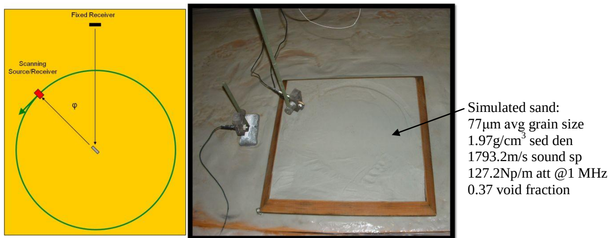
Figure 7. A c-scan track used to collect monostatic and bistatic scattering data from targets deployed on a simulated sand bottom.
