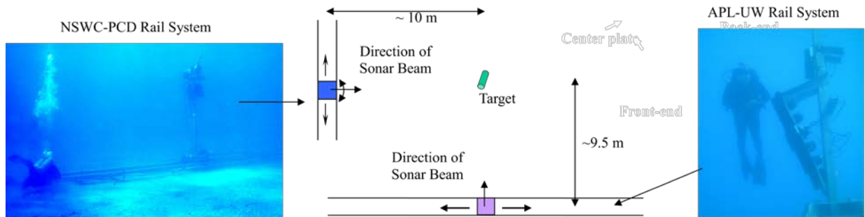
Figure 3. Basic configuration for 2009 shallow grazing angle scattering measurements.
