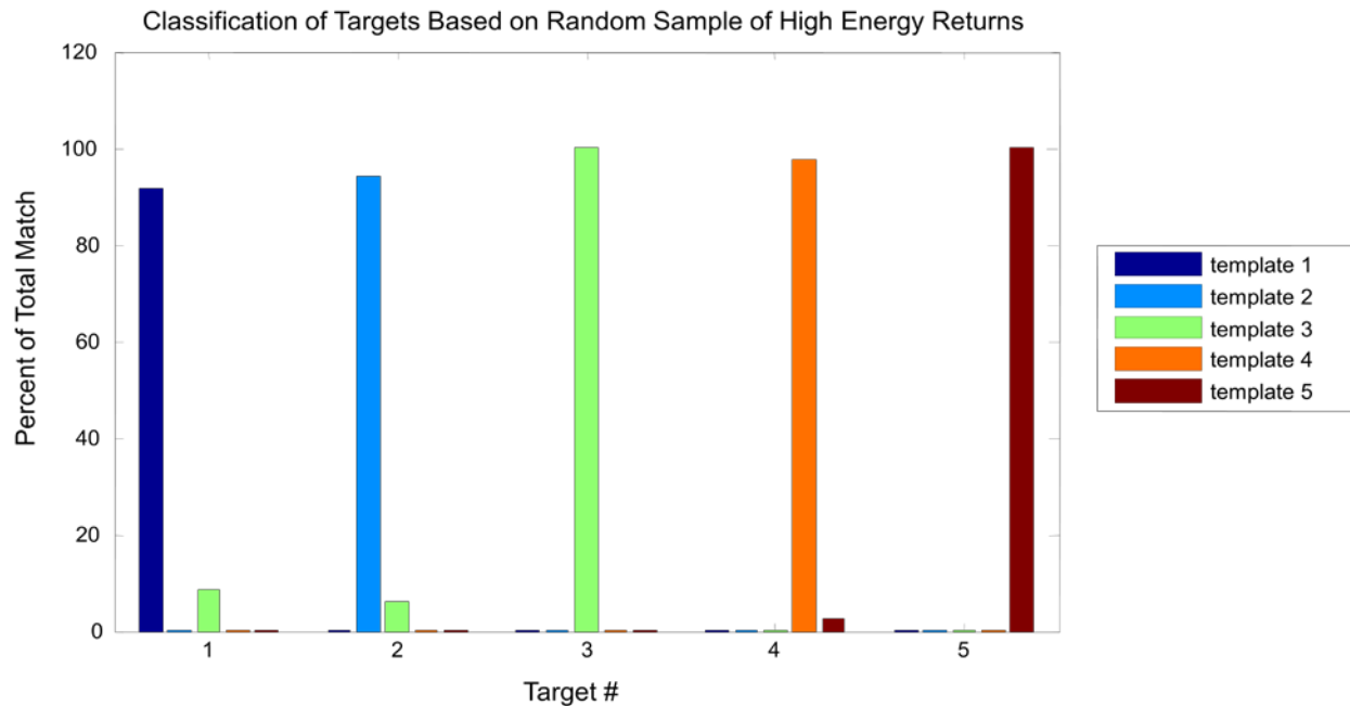
Figure 38. Bar graph demonstrating class separation of data from 5 targets based on templates of high intensity regions in time-frequency space. Percent match is computed as the ratio of the target template area overlapping segment highlights of the test ping to the total target template area. The % match averaged over all 8 pings in the random set is shown above.
