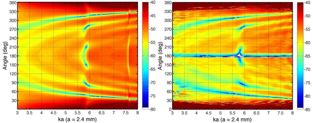
Figure 22. T-matrix simulation model predictions for the target strength (left). Measured bistatic target strength (right).
