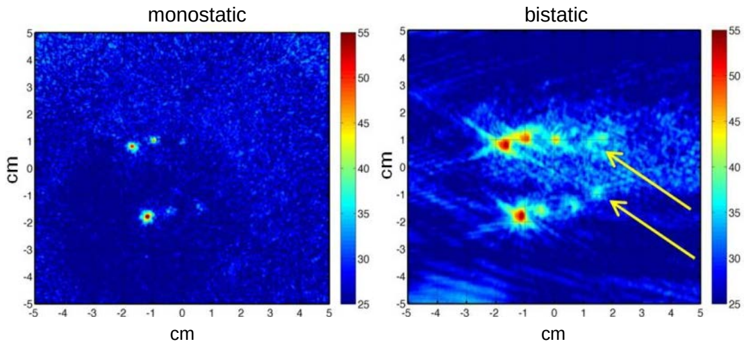
Figure 15. On the left is the monostatic CSAS image resulting from the upper-right time-domain data in Fig. 14. On the right is the bistatic CSAS image resulting from the lower-right time-domain data in Fig. 14. The data are plotted on a dB scale and the amplitudes have not been corrected to account for the different sensitivities of each receiver. As a result, the absolute amplitudes are not comparable between the two images but relative amplitudes against the background (i.e., SNR) may be compared.
