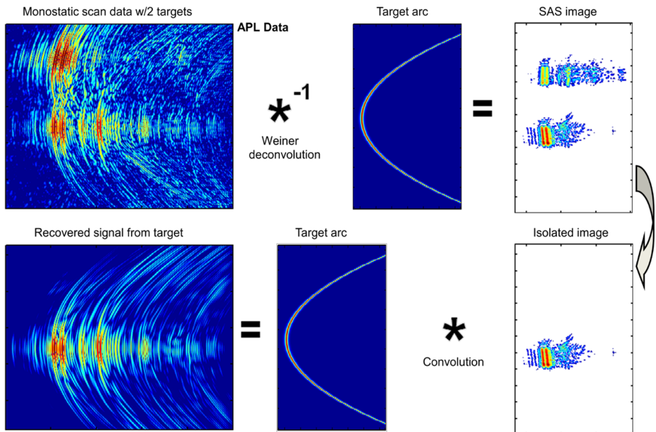
Figure 31. Isolation of selected target signals from noisy data.
