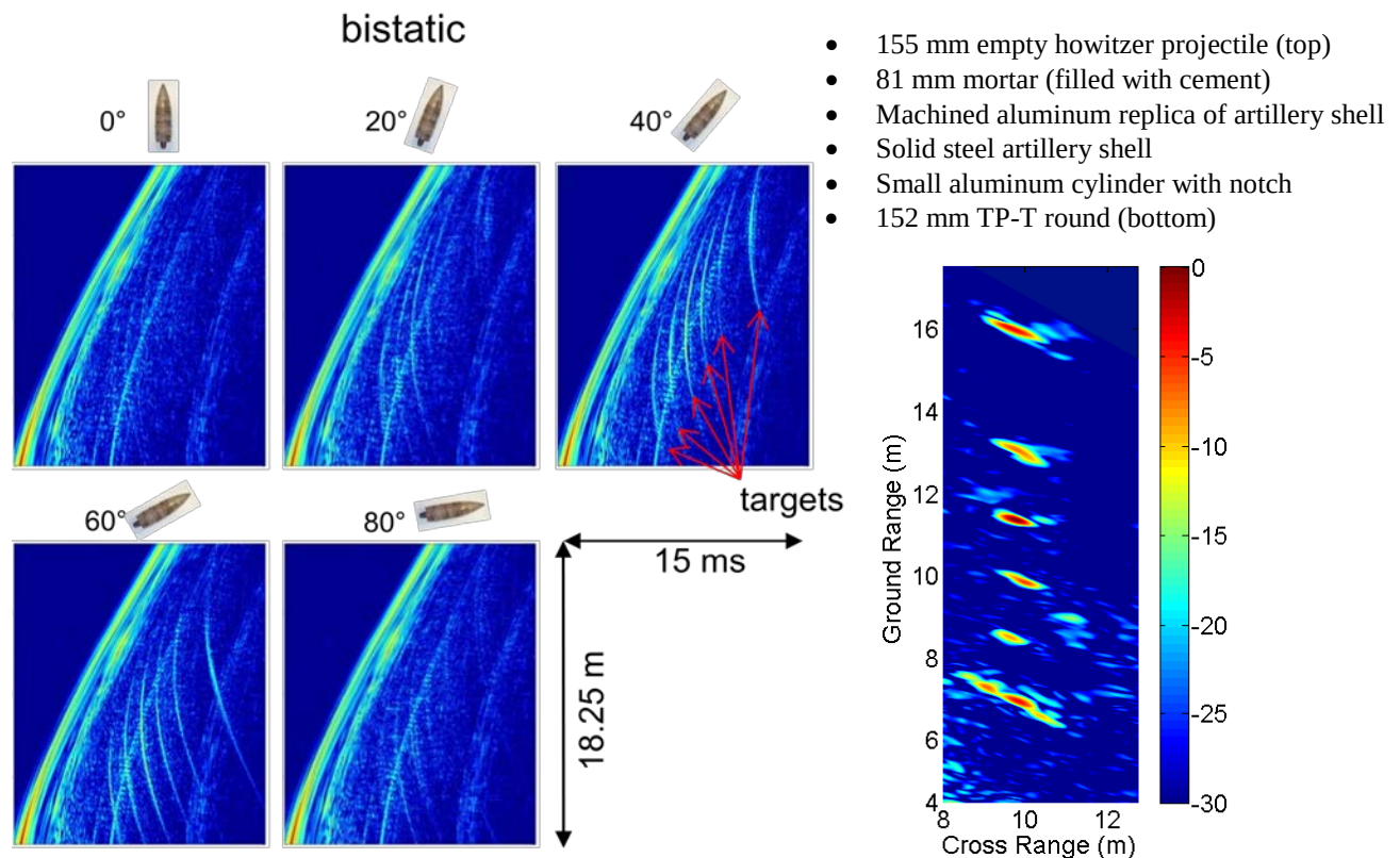
Figure 13. Bistatic target scattering data (left) and processed imagery (right) from 2010 pond measurements.
