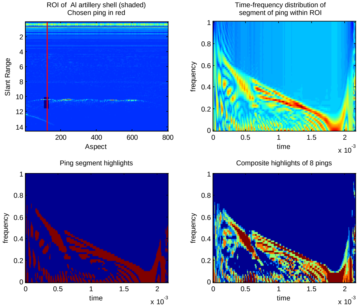
Figure 37. An example of time-frequency processing of data (upper left) collected in NSW PCD's pond facility for the AI artillery shell. The time-frequency transform of a windowed segment of the red ping is shown in the upper right. A thresholded template is shown in the lower left. A composite of 8 templates are overlaid in lower right.
