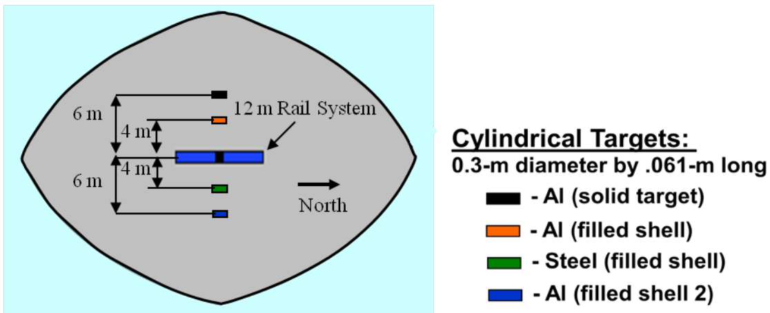
Figure 4. Basic configuration for 2009 high grazing angle scattering measurements.
