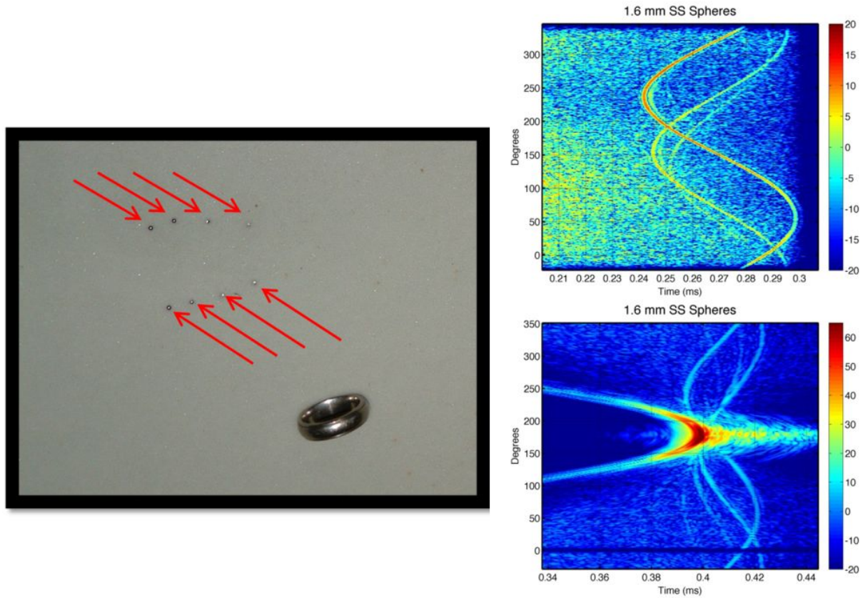
Figure 14. Picture (left) of 8 stainless steel 1.6 mm diameter spheres (red arrows). There is a ring, not present during the experiment, included in the photo to demonstrate the size of the spheres. Monostatic time-series data (upper right). Bistatic time-series data (lower right). The time-domain data are plotted on a dB scale.
