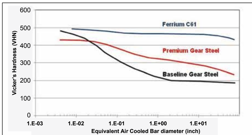
Figure 5—Hardenability comparison for center of an air-cooled bar between legacy baseline steel, current premium grade steel and Ferrium C61.
