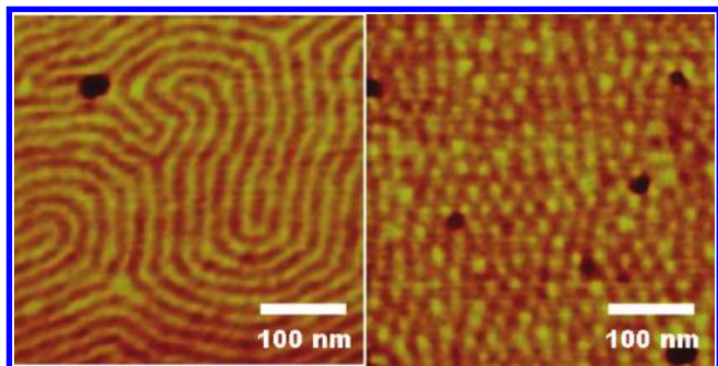
Figure 6. Tapping mode AFM phase images of “dry” films of block copolymers C (left) and S (right), on silicon surfaces.
