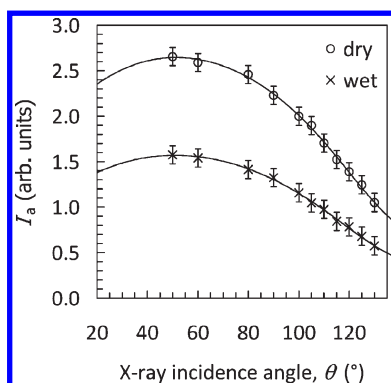
Figure 10. Intensity of the C 1s \rightarrow \pi^*_{C=C} resonance as a function of the X-ray incidence angle for “dry” and “wet” thin films of block copolymer C ; EGB = −150 V. The solid lines are best fit curves for the model discussed in Supporting Information.
