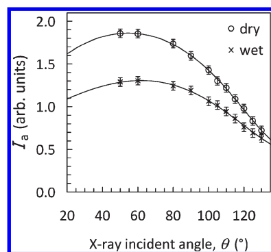
Figure 11. Intensity of the C 1s \rightarrow \pi^*_{C=C} resonance as a function of the X-ray incidence angle for “dry” and “wet” thin films of block copolymer S ; EGB = −150 V.
