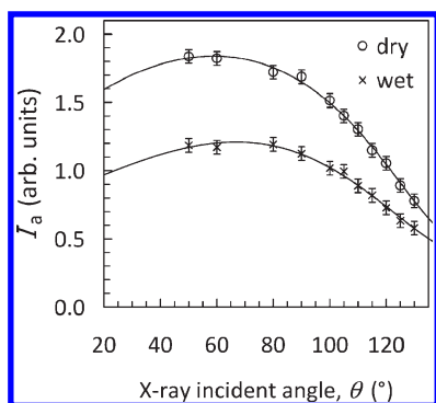
Figure 13. Intensity of the C 1s \rightarrow \pi^*_{\text{C}=\text{C}} resonance as a function of the X-ray incidence angle for “dry” and “wet” thin films of random copolymer R ; EGB = −150 V.
