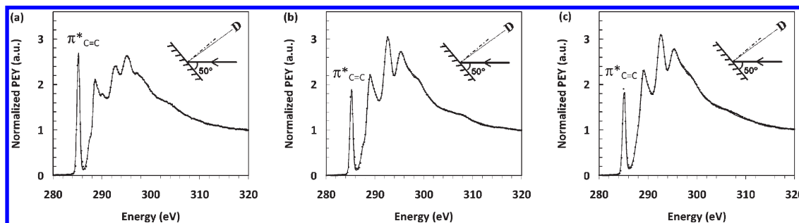
Figure 5. C 1s NEXAFS spectra of surfaces of copolymers (a) C , (b) S , and (c) R , obtained at an X-ray incidence angle of 50°, and an entrance grid bias of −150 V.
