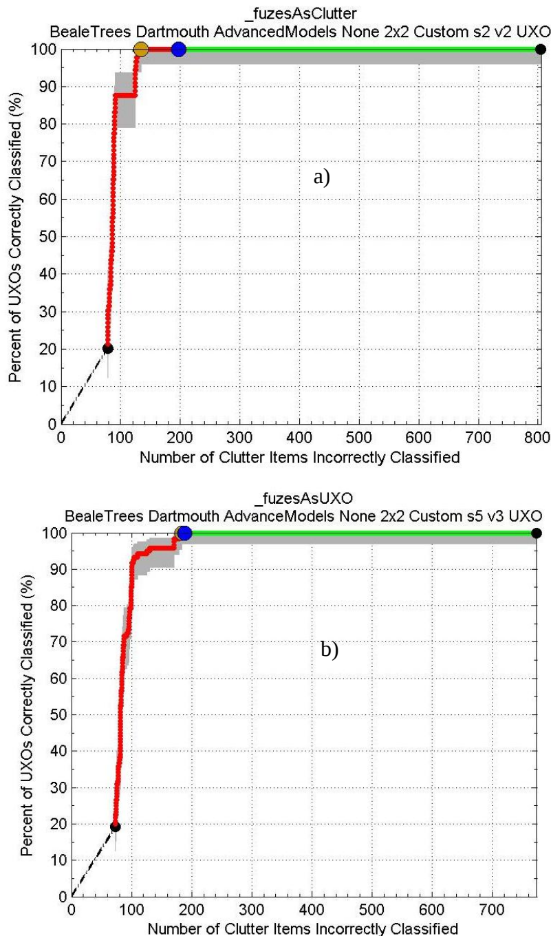
Figure 20. Camp Beale 2 × 2 TEMATDS anomalies ROC curve: a) fuzes as clutter; b) fuzes as TOI.
