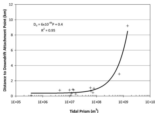
Figure 12. D_d vs. P for 15 highly wave-exposed inlets. The best fit is D_d (km) = 6 \times 10^{-9}P + 0.4 .
