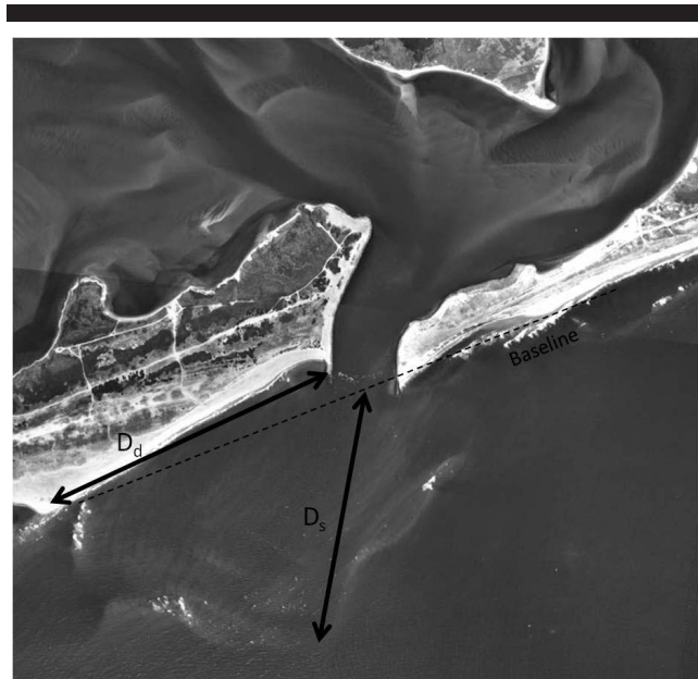
Figure 3. Definition of most seaward extent of ebb delta D_s and the distance to the downdrift attachment bar D_d . Moriches Inlet, New York. Date: 20 March 1995.
