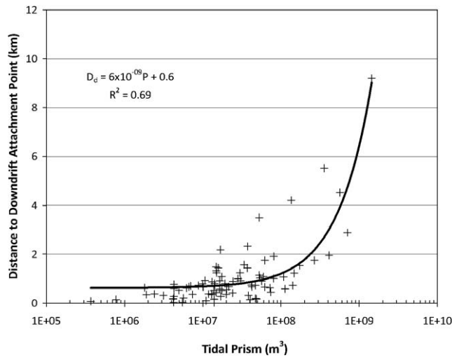
Figure 11. D_d vs. P for 86 inlets in the database. The best fit is D_d (km) = 6 \times 10^{-9}P + 0.6 .
