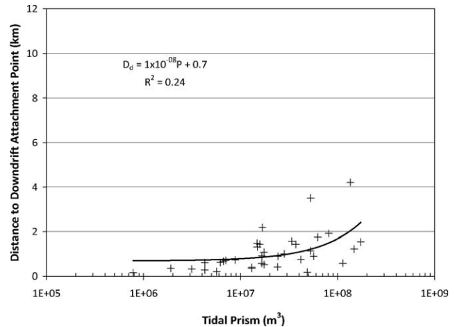
Figure 13. D_d vs. P for 38 moderately wave-exposed inlets. The best fit is D_d (km) = 1 \times 10^{-8}P + 0.7 , with weak correlation.
