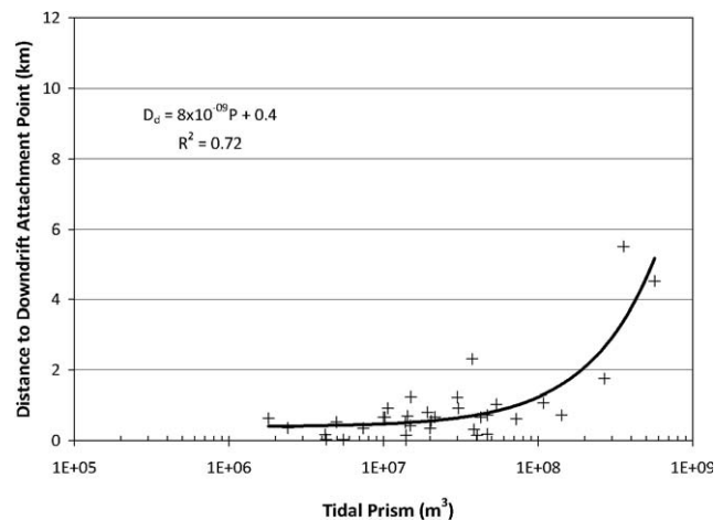
Figure 14. D_d vs. P for 34 mildly wave-exposed inlets. The best fit is D_d (km) = 8 \times 10^{-9}P + 0.4 .
