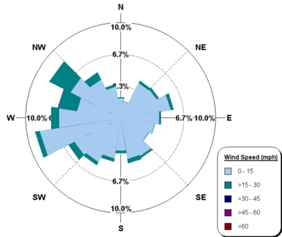
Figure 2. Rose plot of distribution of measured wind speeds from Sandy Hook for the years 1997-99.
