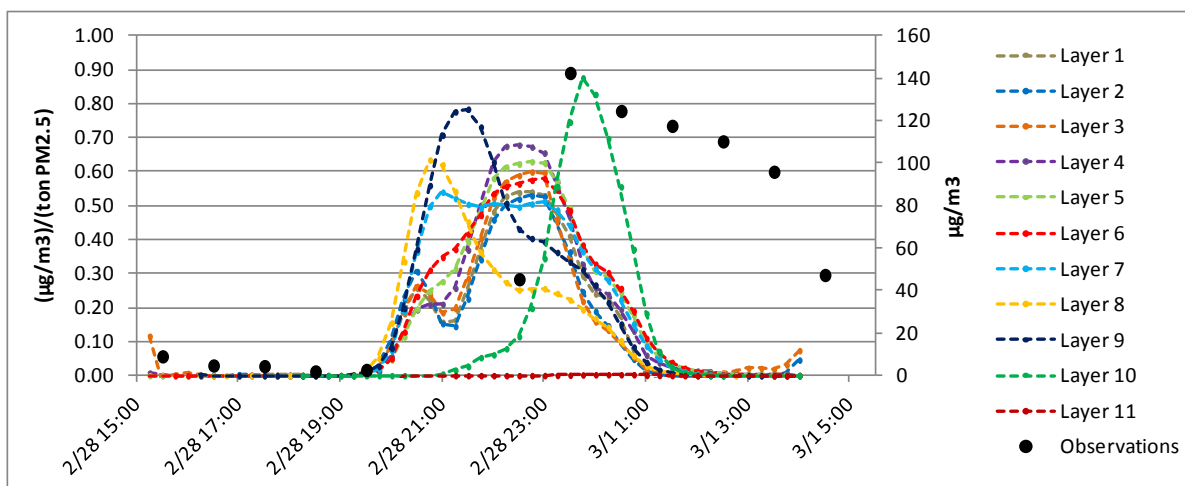
Figure 125. Brute-force sensitivity coefficients for PM 2.5 concentration response to fire emissions by vertical CMAQ layer at South DeKalb (left axis) and site observations (right axis). Time is UTC.
