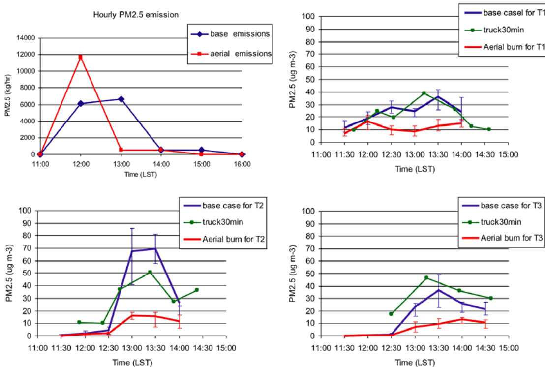
Figure 136. Effects of ignition type: aerial vs. hand lit. Comparison of input emissions (top left) and downwind PM 2.5 concentrations at 2 miles (top right), 3.5 miles (bottom left), and 5 miles (bottom right) from the fire.
