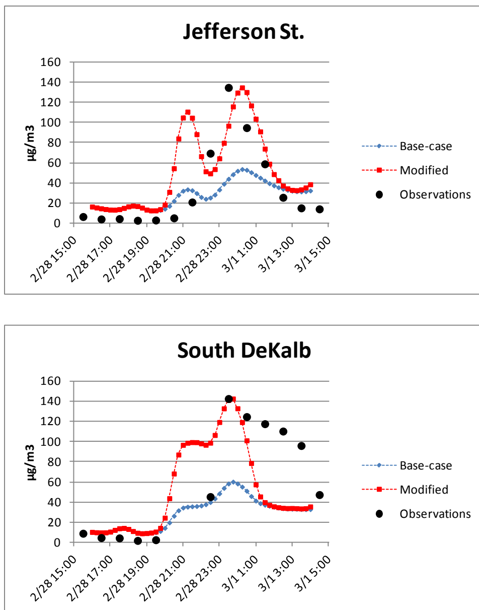
Figure 120. Base-case and modified CMAQ-predicted PM 2.5 concentrations along with monitoring site observations. Fire emissions for modified simulations were increased by factors of 5.1 (Jefferson St.) and 3.7 (South DeKalb). Time is UTC.
