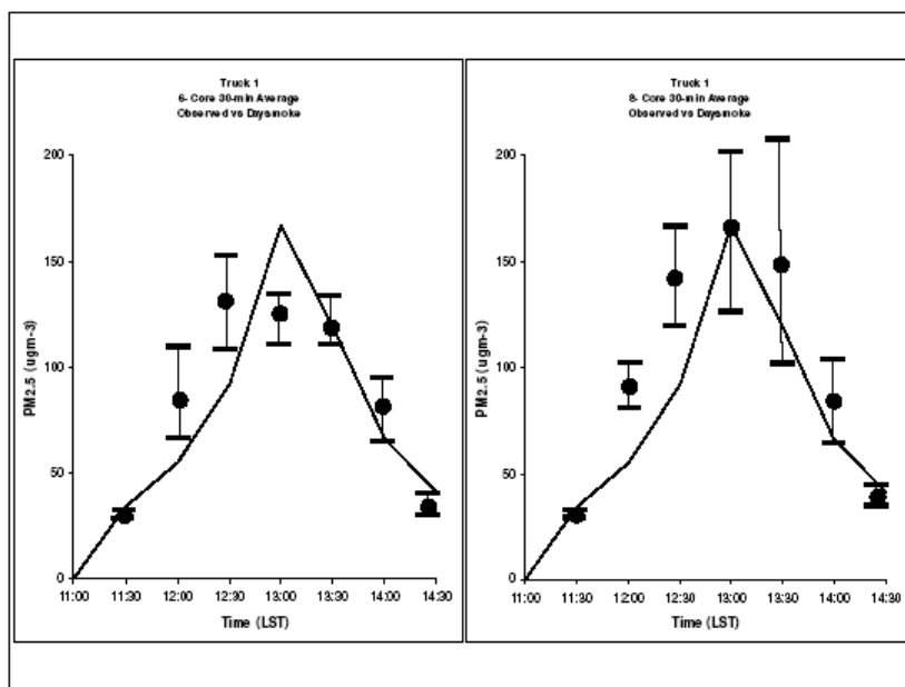
Figure 73. 30-min averaged PM 2.5 generated by Daysmoke for 6-core updraft plumes (left panel) and 8-core updraft plumes (right panel) compared with 30-min averaged observed PM 2.5 at the Truck 1 locations during 9 April 2008 burn at Fort Benning.
