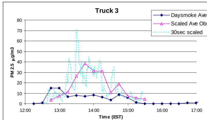
Figure 83. Modeled versus measured PM 2.5 concentrations at truck locations. Modeled concentrations are the average of 5 Daysmoke runs using 4 updraft cores. Measured concentrations are DustTrak readings scaled by a factor of 27.5%.
