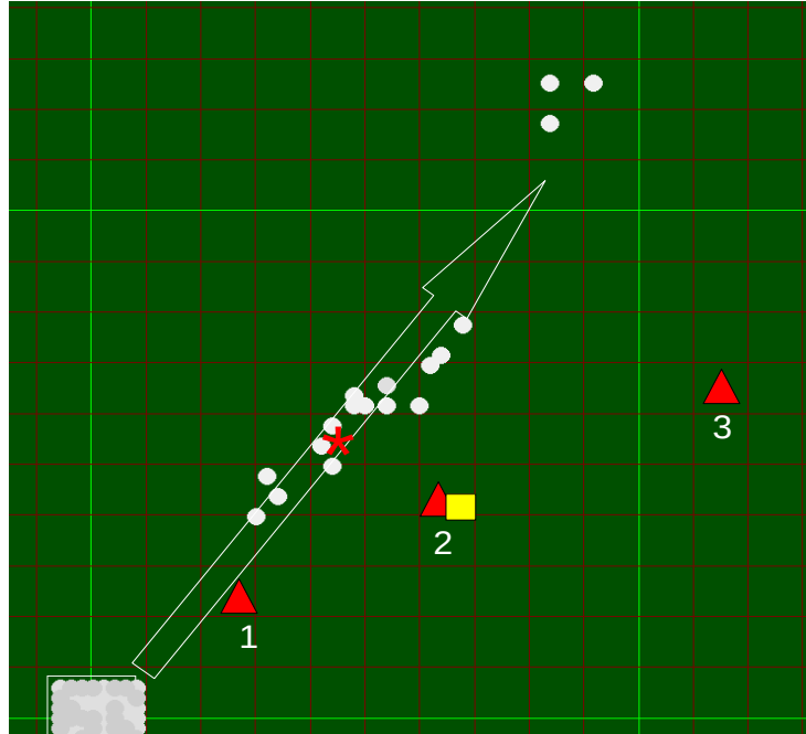
Figure 106. Ground-level \text{PM}_{2.5} average concentrations simulated by Daysmoke for a 2-hr period beginning at ignition of the 6 February 2011 burn in Block 703C at Eglin AFB, using the MM5 meteorological sounding. The white dots indicate above-background concentrations due to smoke of 1\text{--}2\ \mu\text{g m}^{-3} . The small squares represent 1 mi (1.6 km) and the light green square represents 10 mi (16 km). The axis of the plume is given by the white arrow. Also shown are locations of the ceilometer (yellow square) and three \text{PM}_{2.5} sampling units (red triangles).
