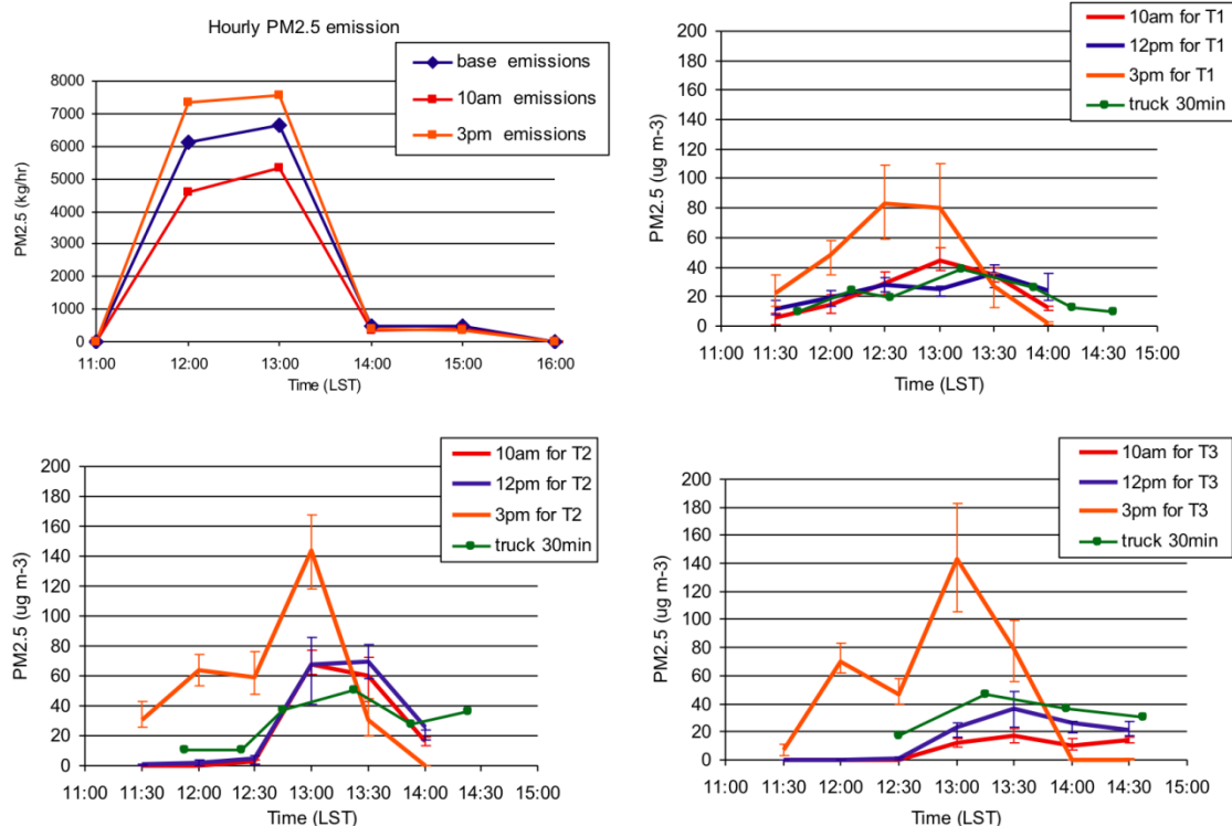
Figure 137. Effects of time of burn: morning and afternoon vs. noon. Comparison of input emissions (top left) and downwind PM 2.5 concentrations at 2 miles (top right), 3.5 miles (bottom left), and 5 miles (bottom right) from the fire.
