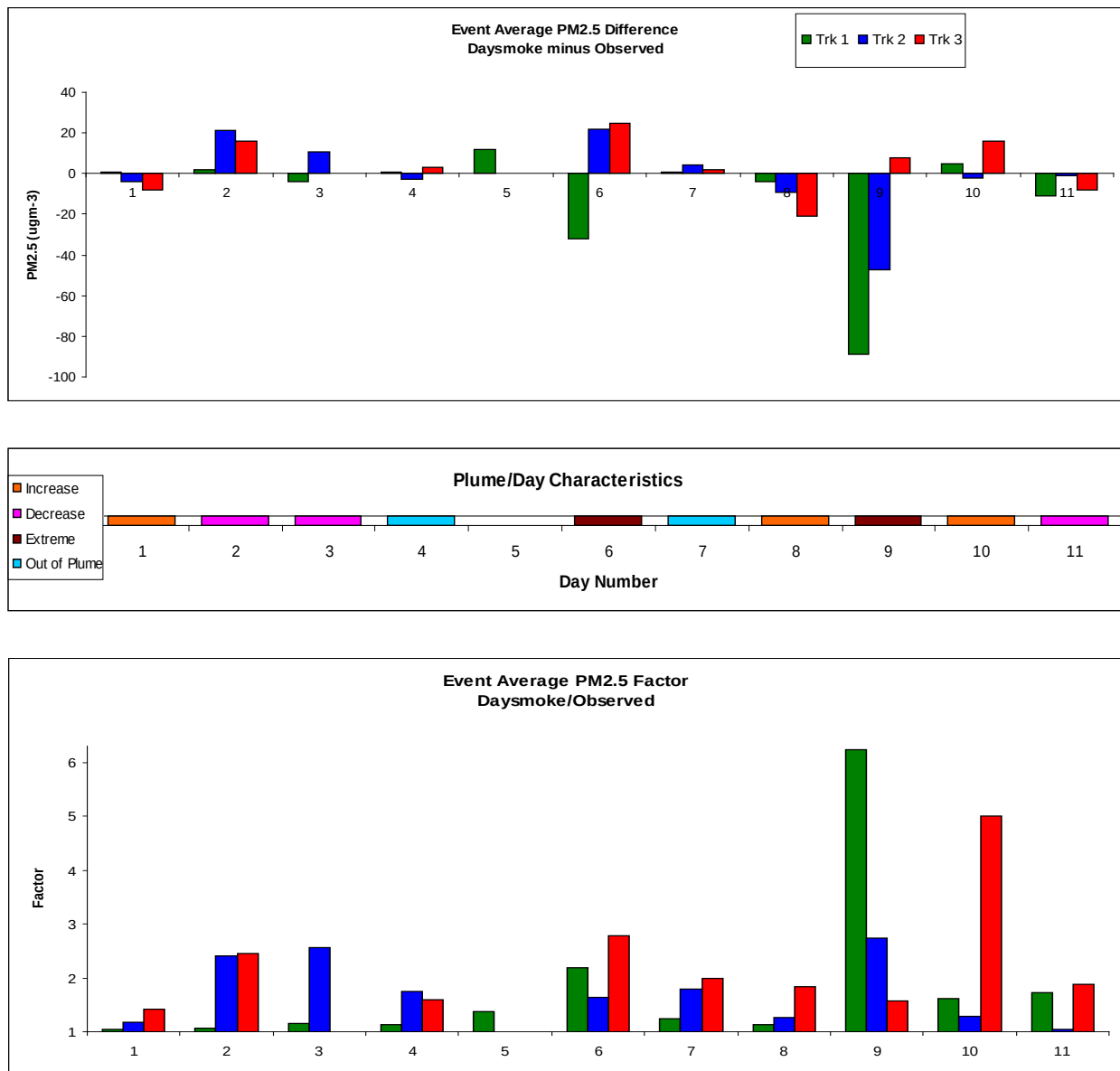
Figure 99. Daysmoke performance for each burn event and at each monitor: difference of modeled PM_{2.5} from observed (top), classification of the burn event by the trend of concentration with distance downwind (middle), and ratio of modeled to observed or vice versa PM_{2.5} (bottom).
