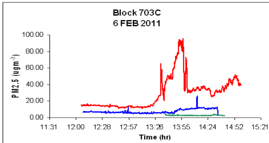
Figure 107. Measurements of \text{PM}_{2.5} taken at the three sites in Figure 106: Site 1 (red), Site 2 (blue) and Site 3 (green).
