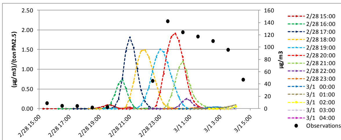
Figure 129. Brute-force sensitivity coefficients for \text{PM}_{2.5} concentration response to fire emissions by hour of emissions at South DeKalb for uniform distribution into 10 lowest layers (left axis), and site observations (right axis). Emissions are labeled at the start of the hour. Time is UTC.
