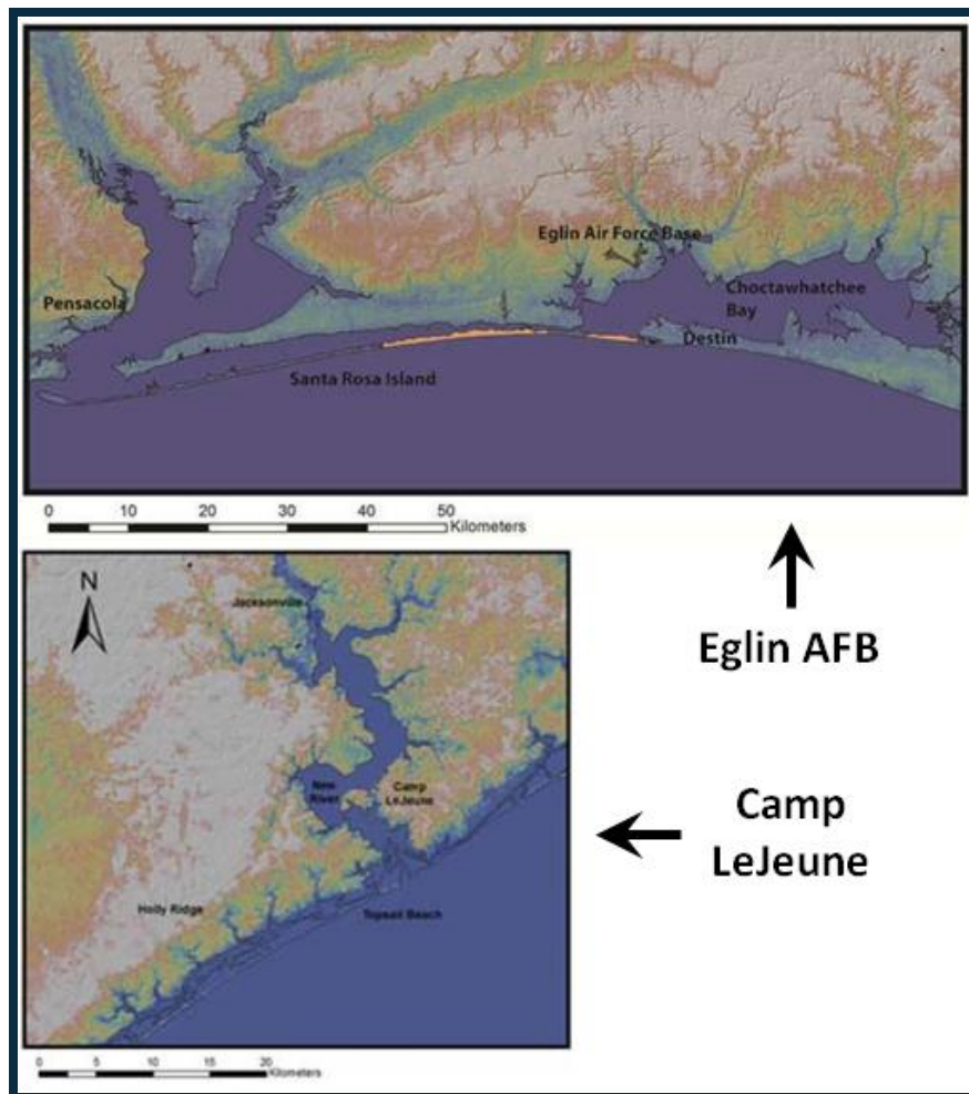
Figure 5: Focus Areas of Shoreline Evolution Study.
