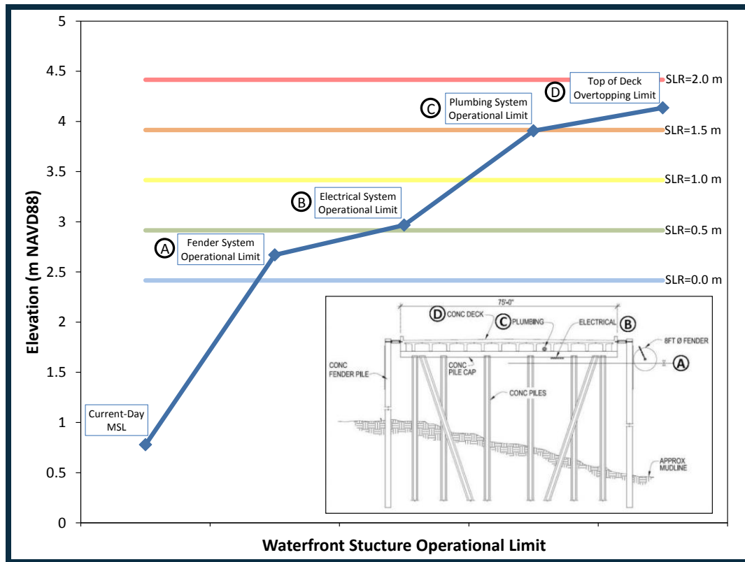
Figure 11: Coastal military installation infrastructure has unique damage response characteristics.
