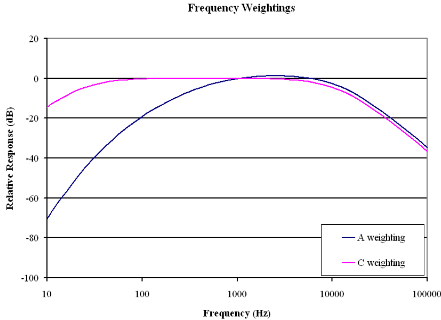
Figure A 1. A and C Frequency Weighting Characteristics. vi
