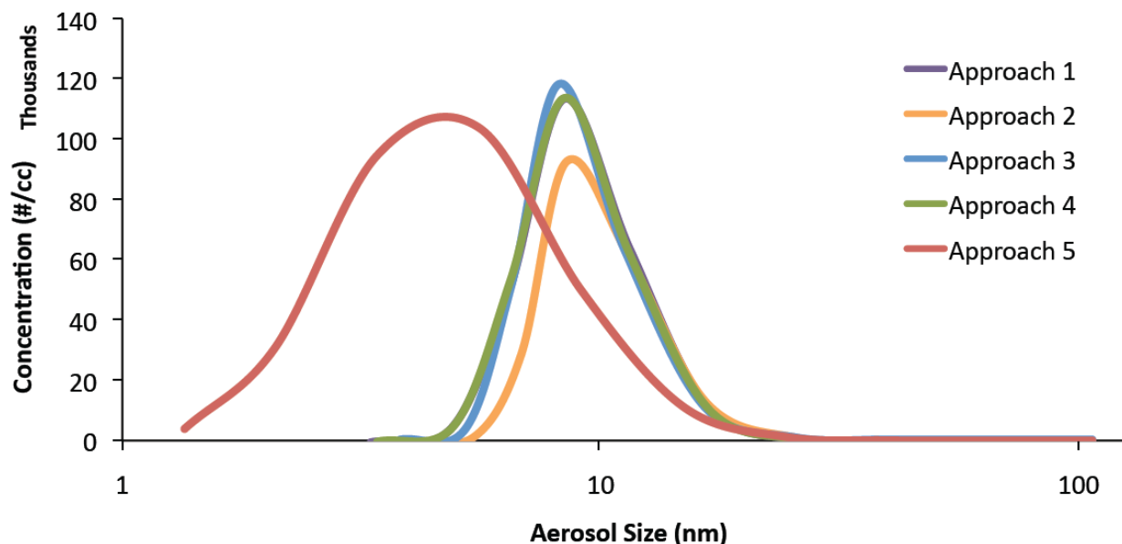
Figure 2.16 Comparison of predicted particle size distributions of liquid aerosols at 1 km downstream of a CFM56-2C1 engine by involved different interactions in nucleation and coagulation processes
