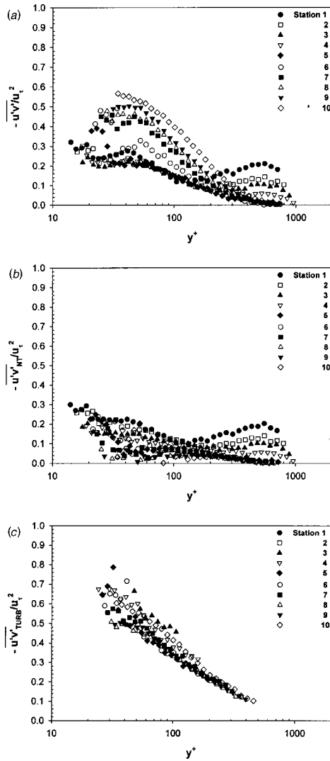
Fig. 15 Reynolds shear stress profiles in wall coordinates: (a) composite; (b) nonturbulent; (c) turbulent
