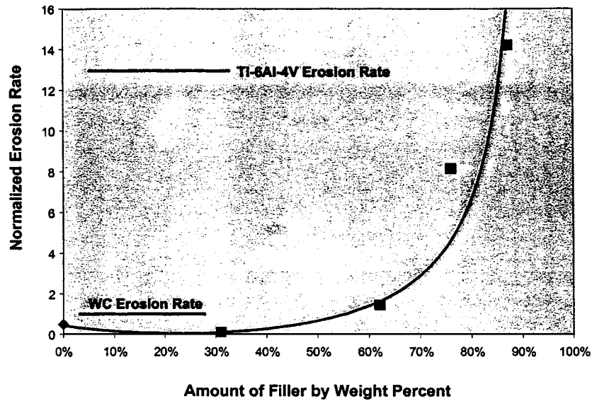
FIGURE 7 Effect of filler on erosion of ECN-A coatings.
