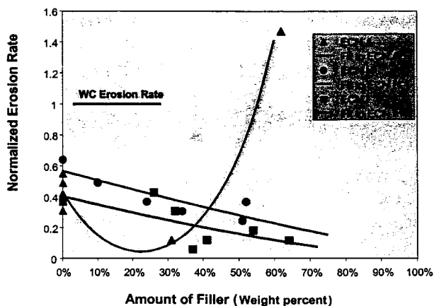
FIGURE 8 Effect of improved filler-to-matrix interface in ECN-H and ECN-I coatings on the erosion rate.
