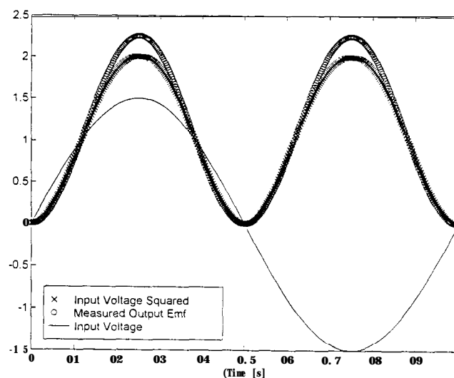
Figure 1. Comparison between measured output E_{cmf} -o-, and input voltage squared, -x-.
