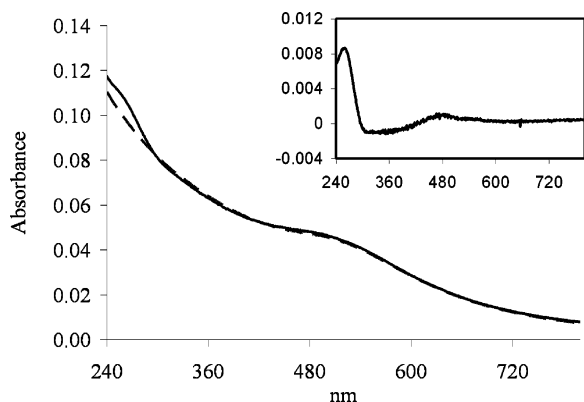
Figure 3. UV-vis spectra of solutions of (a) AuEO3 (---) and (b) AuEO3-DNA isolated by extraction (—). Inset: background subtracted spectrum (b – a) used for quantifying DNA.
