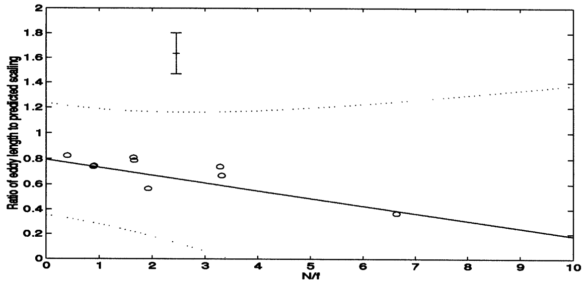
Figure 3.8: Laboratory values for normalized eddy length ( \frac{l_{eddy}^{lab}}{l_{eddy}^{scal}} ) plotted against N/f .
