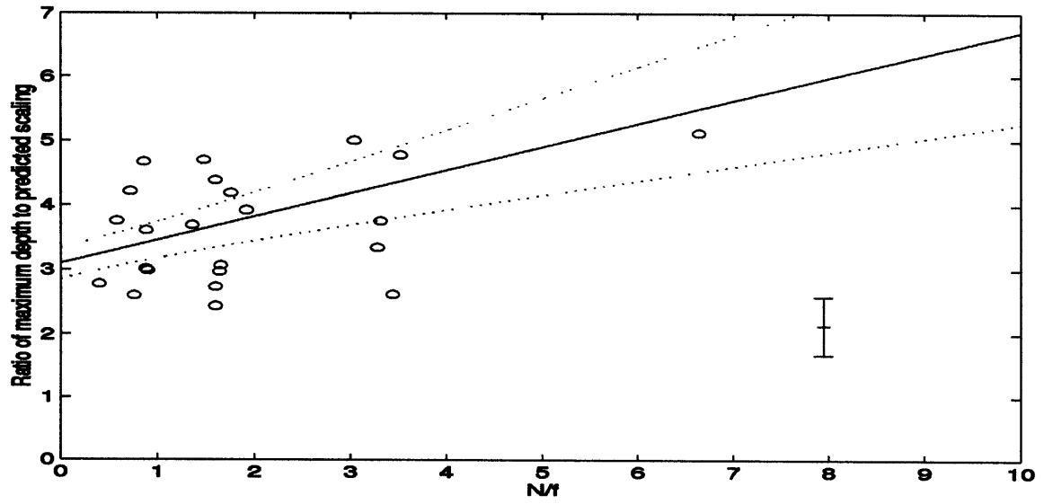
Figure 3.10: Laboratory values for normalized maximum depth ( \frac{d_{max}^{lab}}{d_{final}^{scal}} ) plotted against N/f .
