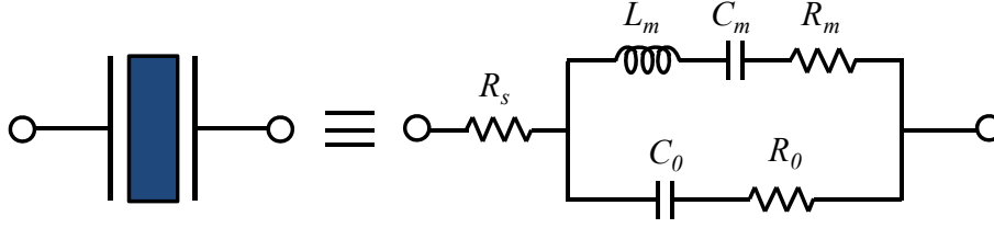
Figure 3-10. Modified Butterworth-Van Dyke (MBVD) equivalent circuit for a piezoelectric resonator.
