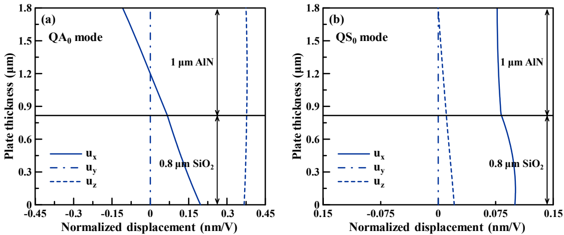
Figure 2-11. Normalized displacement profiles to surface potentials of the (a) QA 0 and (b) QS 0 Lamb wave modes in an AlN/SiO 2 multilayer plate while h_{\text{AlN}} is 1 \mu\text{m} and h_{\text{SiO}_2} equals 0.8 \mu\text{m} .
