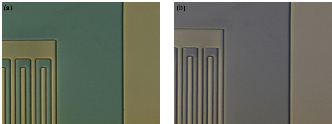
Figure 4-10. Microscope images of the Al top electrodes with 20-nm-thick Nb after (a) 400-nm-thick PECVD oxide deposition and (b) then 2-μm-thick LPCVD LTO deposition.
