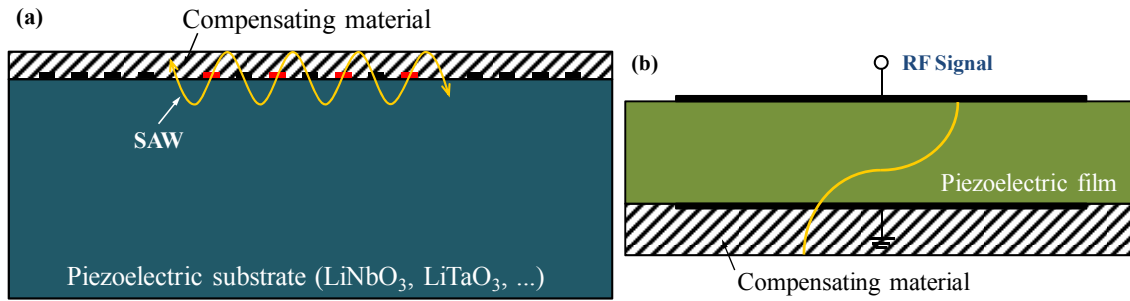
Figure 1-12. Illustrations of passive temperature compensation for (a) SAW and (b) BAW resonators.
