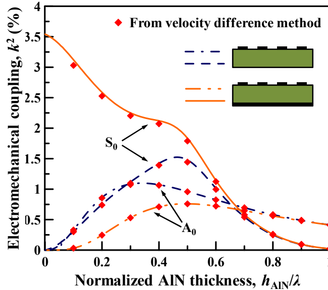
Figure 2-7. Comparison of k^2 computed from the Green's function with the velocity difference method.
