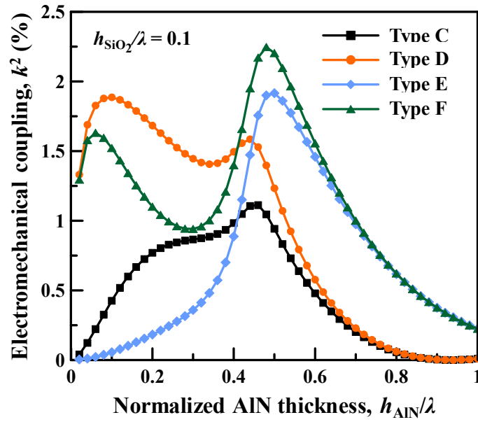
Figure 2-13. Comparison of k^2 of various types of AlN/SiO 2 LWRs while the h_{\text{SiO}_2} is equal to 0.1\lambda .
