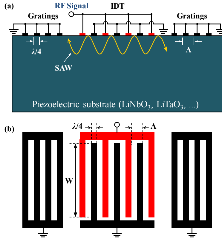
Figure 1-5. (a) Cross-sectional illustration and (b) top view of one-port SAW resonator.
