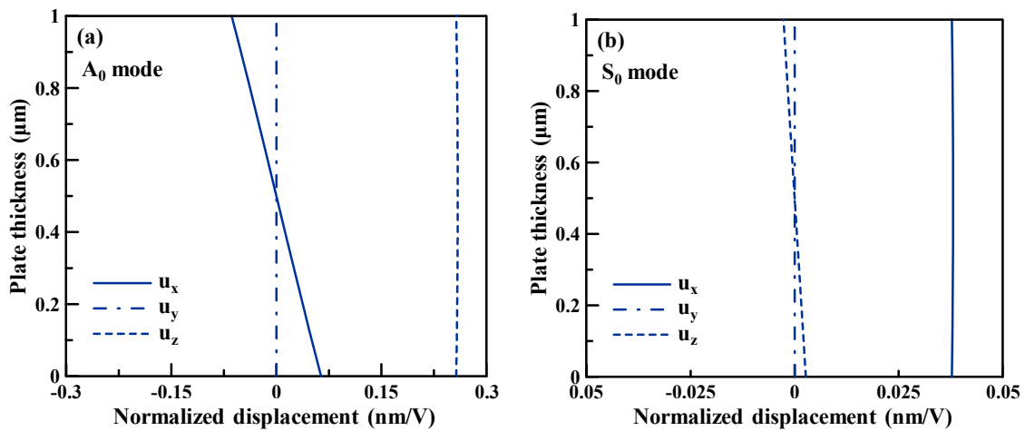
Figure 2-5. Normalized displacement profiles to surface potentials of the (a) A_0 and (b) S_0 Lamb wave modes in a 1- \mu\text{m} -thick AlN plate.
