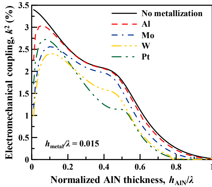
Figure 3-3. Simulated electromechanical coupling of the S_0 mode in AlN films with various bottom metals while the metal thicknesses normalized to the wavelength are fixed to 0.015.
