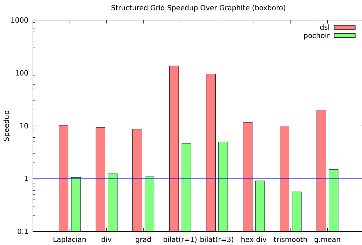
Figure 10.9: Performance for single-iteration kernels on Boxboro.
