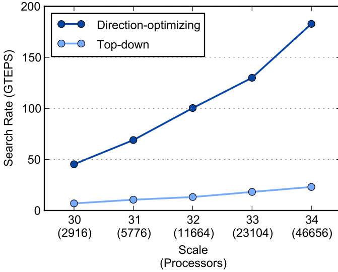
Fig. 2. R-MAT weak scaling on Jaguar
