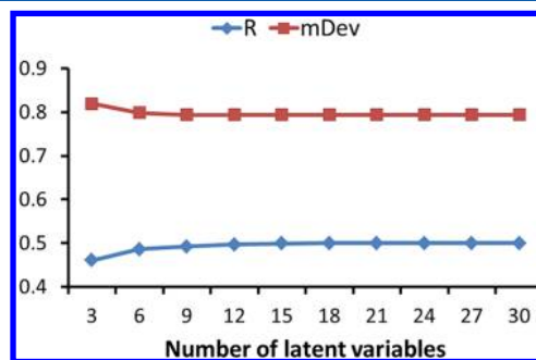
Figure 6. Performance of partial least-squares regression with different number of latent variables as measured by R and mDev values between the predicted and database log(MRDD) values obtained from 40-fold cross-validation using the FDA MRDD training set.
