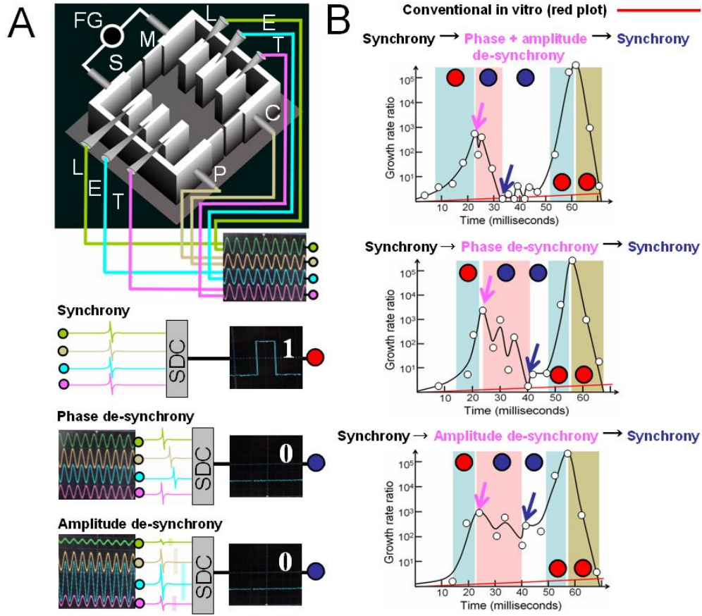
Figure 2: Switching between synchrony and de-synchrony to switch between two kinds of in vitro processes: A. Replica of living cell, with PCMS ion gates and heat bath at 37 0 C, cell dimension of Figure 2A fixed for all species (200 \mu m), two 200nm ion-channels. FG is function generator, and connected circuit is the ac pumping circuit. L, E, T signals and two cables from PCMS is connected to oscilloscope. Signals of synchrony is demonstrated on top, phase de-synchrony in the middle and amplitude de-synchrony is at the bottom. An AND gate inside SDC checks whether signals arrive at same time, or same amplitude if “yes” we see “1” in the oscilloscope, and if “no” then “0”. B. Growth rate is switched off by disrupting synchrony in three ways, de-synchronizing both phase and amplitude, (top), de-synchronizing only phase (middle), and desynchronizing only amplitude (bottom) by sending noise into the solution. Pink arrow shows when noise is applied to de-synchronize. Blue arrow shows when noise is off and synchrony recovers slowly. Once microtubule nucleates from tubulin, silent mode is not distinctly visible, hence recovery to synchrony is fast. Growth rate ratio means Growth rate for tubulin density at higher than natural synchrony to growth rate at lower tubulin density.
