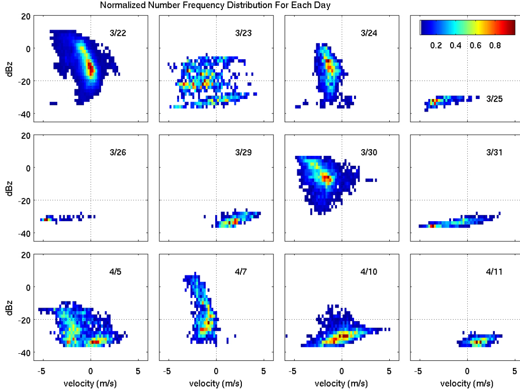
Fig. 2. Normalized velocity-reflectivity number frequency distribution on each day during BACEX. Color bar is shown in upper right corner. Reflectivity of -20 dBz and Doppler velocity of 0 m s ^{-1} are denoted by dotted line. No clouds are observed on 1-2 April during the cloud-base level flights.
