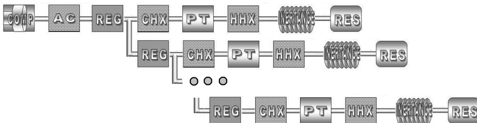
FIGURE 2. Multistage ITPTR – each subsequent stage is usually at a colder temperature than the previous stage.
