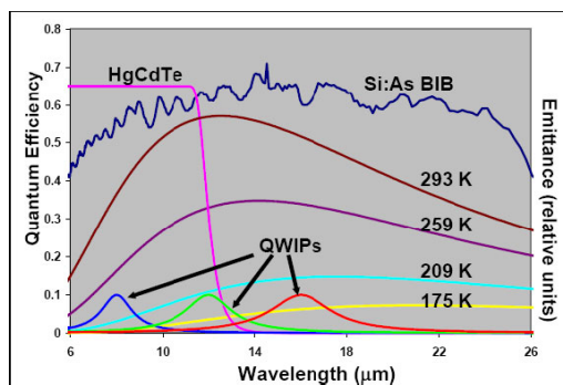
Figure 7. Performance curves of Selected FPA Materials
