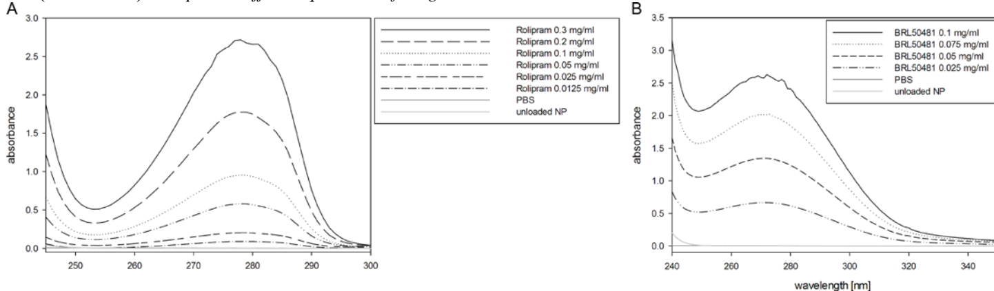
Fig.9: Absorbance spectra of Rolipram (A) and BRL50481 (B).
