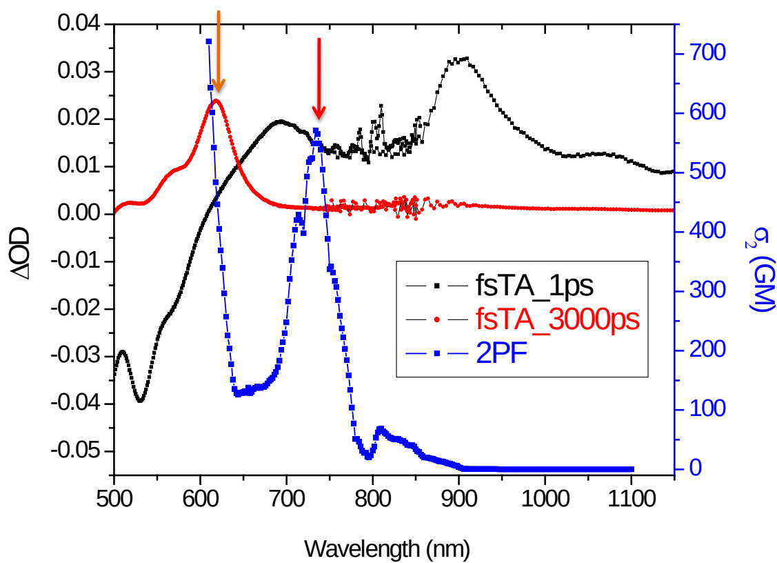
Figure 20: Two-Photon Absorption and fs-Transient Absorption Spectra of HxThio in Toluene.
