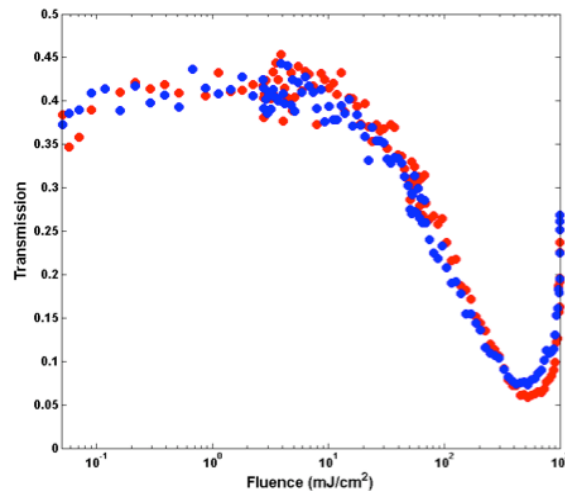
Figure 22. Transmission through 24 layer nonlinear mirror made from PVK and \text{Co}_3\text{O}_4 -doped PVA
