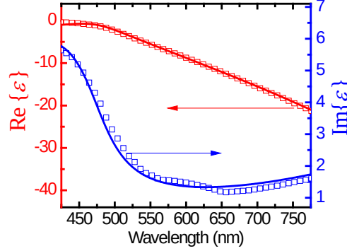
Fig. 1 Comparison of measured (symbols) and simulated (solid lines) complex dielectric permittivity spectra in visible range for fabricated samples R1 . The dielectric permittivity of Au was modeled as a set of explicit equations (Eqs. 2-4) and compared with measured ellipsometric data.
