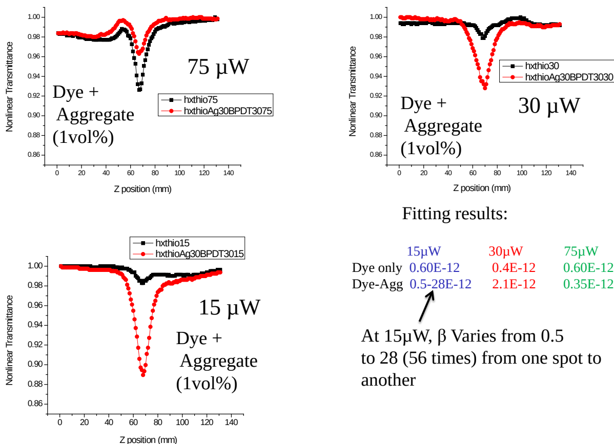
Figure 23: The z-scan traces of the HxTHio+Ag aggregates at different power.
