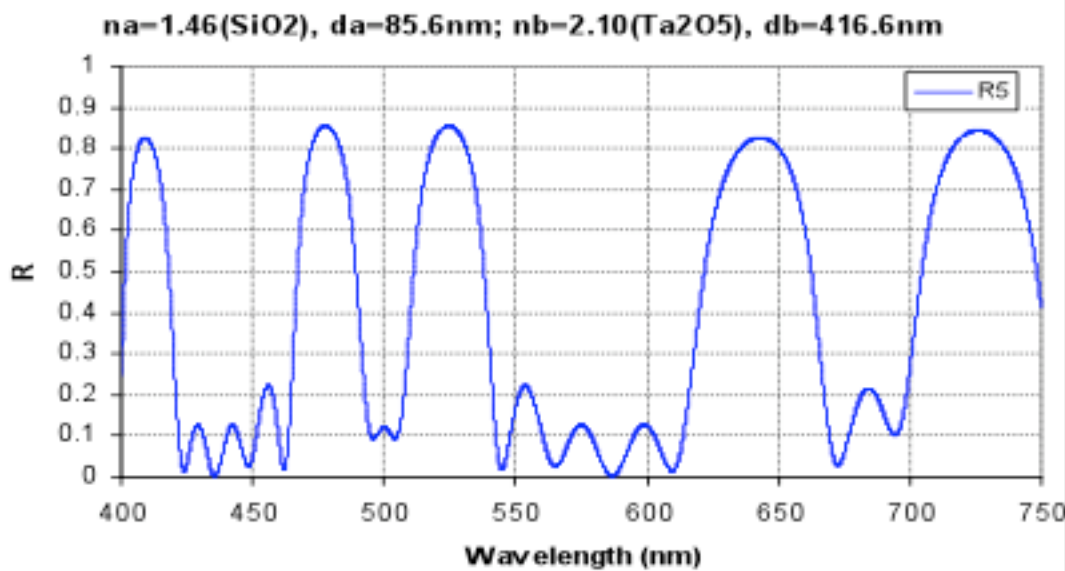
Figure 32. Designed spectral performance of multiple window Fibonacci mirror
