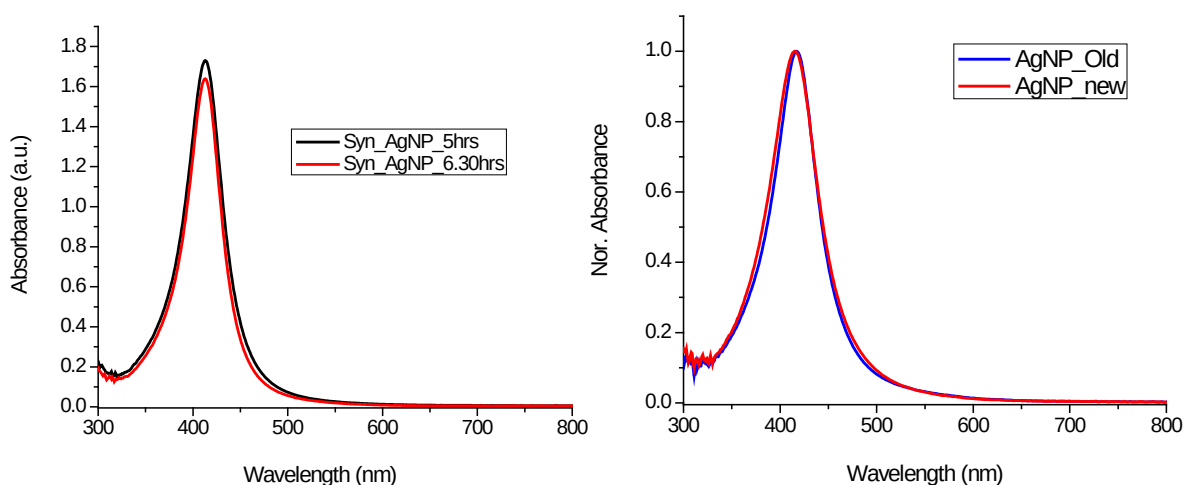
Figure 21: Synthesis of oleylamine-capped AgNP followed by absorption spectra (left after 5 and 6.30 hrs after the starting of the reaction). The right spectra show the reproducibility of the AgNP synthesis.
