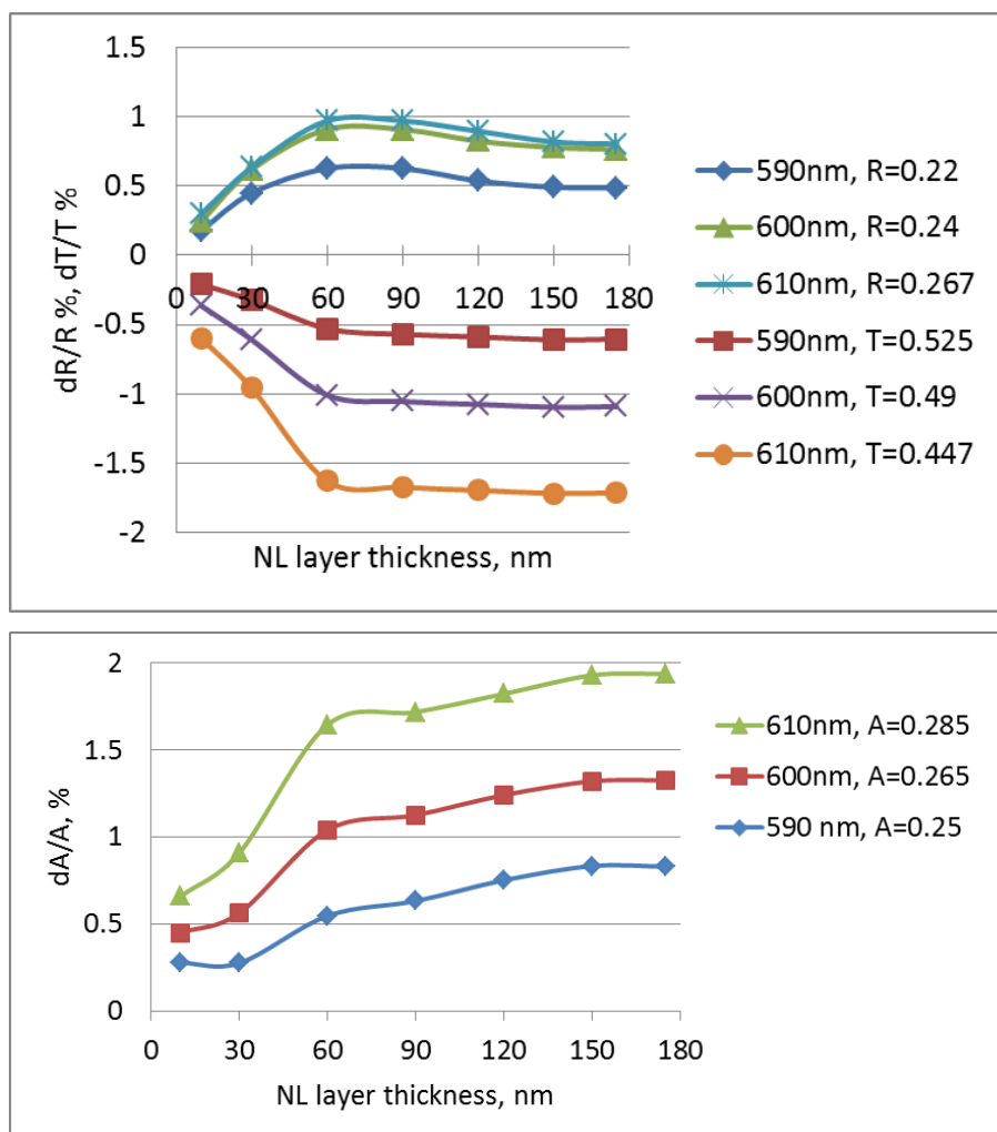
Fig. 5.3 Relative nonlinear changes (%) in transmission ( dT/T ), reflection ( dR/R ) (upper panel), and absorption ( dA/A ) at three wavelengths 610, 600, 590 nm; the linear values of T, R, A are shown in the legends as a fraction of unity.
