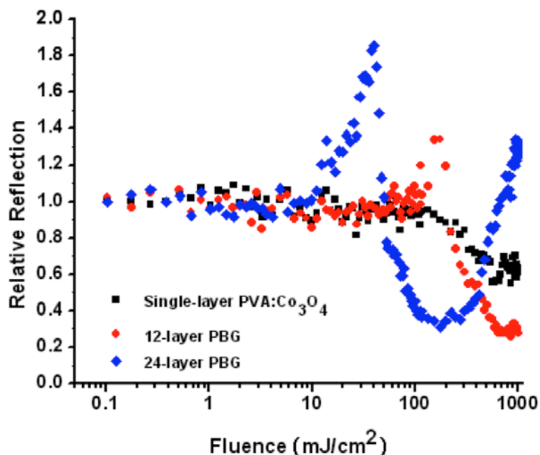
Figure 30. Relative reflection of single layer film, 12-layer PBG, and 24-layer PBG as function of fluence
