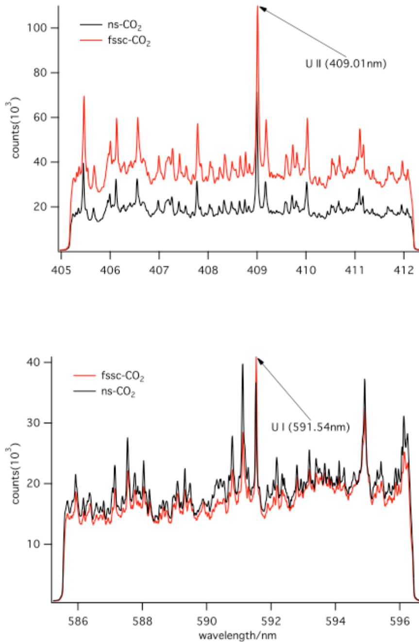
Figure 2. Comparison of CO 2 enhancement for nanosecond and femtosecond produced plasma for U II (409.01nm) and U I (591.54nm) emissions
