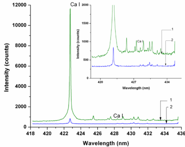
Figure 67. Enhancement difference between different Ca lines.
