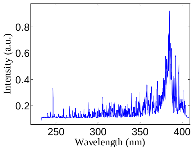
Figure 90. Single-shot. LIBS spectrum from graphite at 400 meters.
