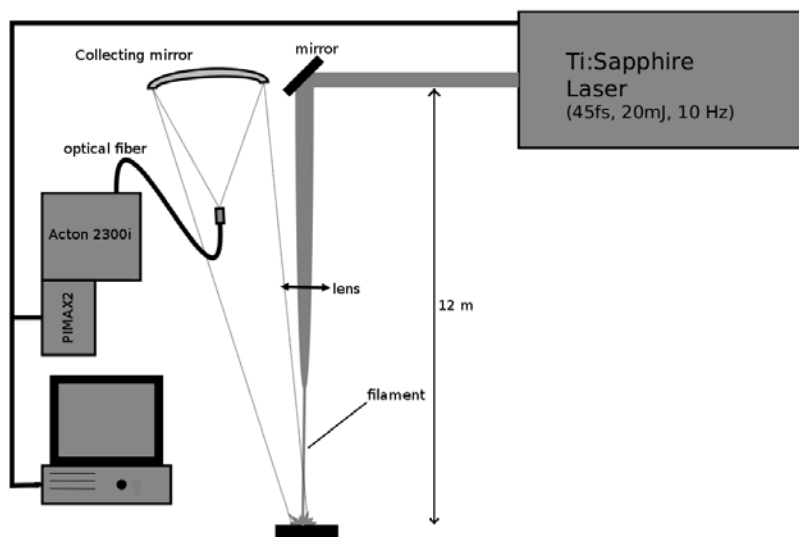
Figure 81. Experimental setup.
