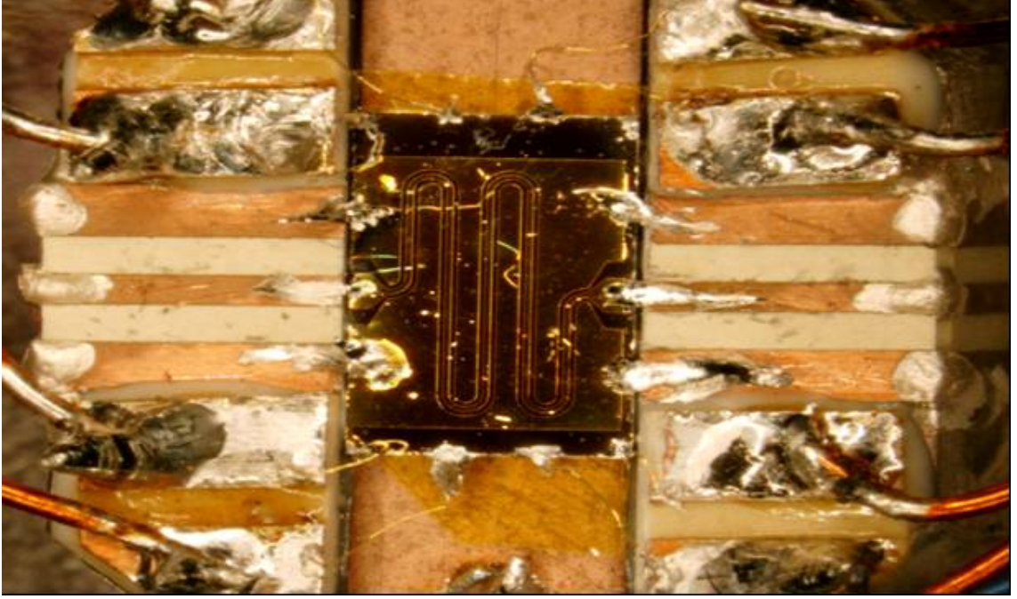
Figure 2.4: Picture of a sample mounted on a block. The sample is \sim 3 \times 5 mm in size and is equipped with a CPW (“M60”) of l=15.5 mm and slot w=60 \mu\text{m} . The CPW on the sample is joined by “indium bridges” to the circuit-board CPW on the block. The circuit board CPW further mates (mechanically via pressed pins) to the semirigid coax at the side of the block (not shown). Also seen are (gold) DC wires making connection to the (indium) ohmic contacts on the sample.
