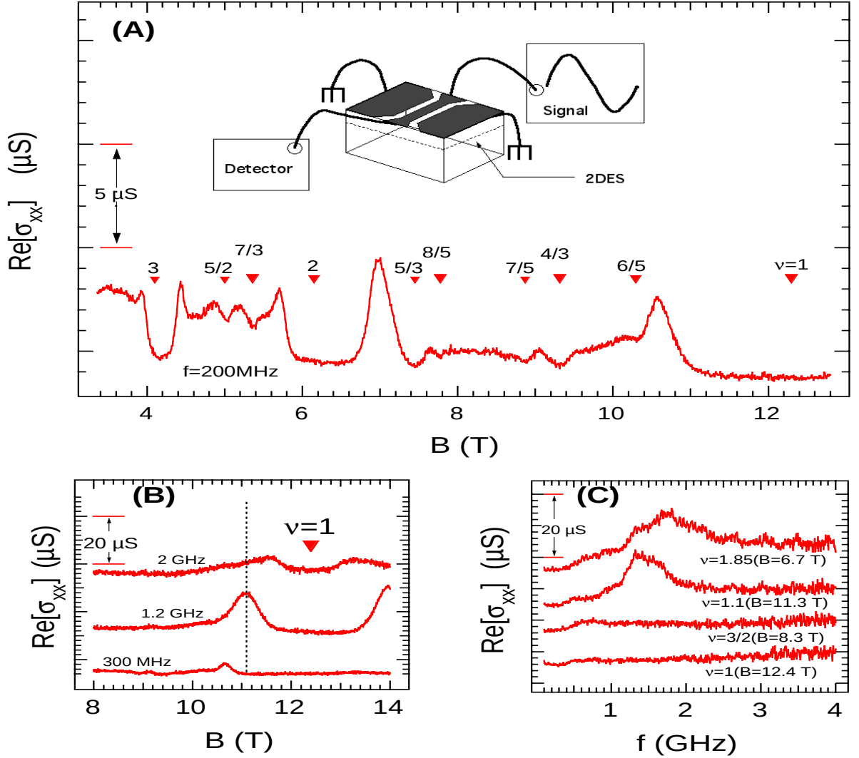
Figure 4.1: Sample R, overview near integer fillings. (A) The B -dependent conductivity at 200 \text{ MHz} and \sim 80 \text{ mK} with a slightly elevated microwave power. Several filling factors are marked. Inset shows the schematic measurement circuit. Dark regions represent the metallic films deposited on the sample to make the CPW. (B) B -dependent conductivity around \nu = 1 measured at three different frequencies as labeled. Traces appropriately offset vertically for clarity. The temperature during B -sweep is about 80 \text{ mK} . Dotted line is a guide to the eye for the resonating behavior. (C) A few f -dependent conductivity spectra (offset for clarity) measured at \sim 50 \text{ mK} and at various B fields labeled underneath each trace. Data in both panel B and panel C are measured with a low microwave power.
