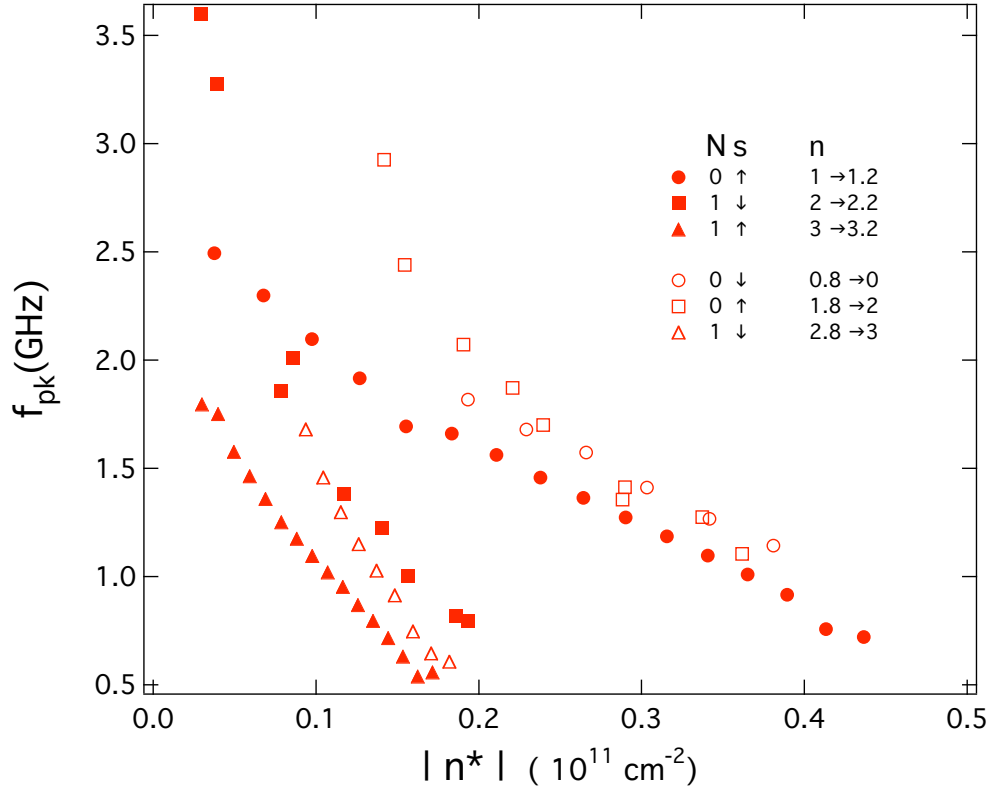
Figure 4.6: Summary of f_{pk} (of the resonance shown in Figs. 4.2,4.3,4.4) vs n^* (of partially filled top LL). N is the orbital LL index and \sigma the spin index. The solid symbols indicate IQHWC of Landau-electron, and empty symbols for IQHWC of Landau-holes. All data measured in Sample R at \sim 50 mK.
