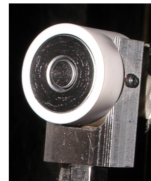
Faraday Probe (22 mm outer dia.)
