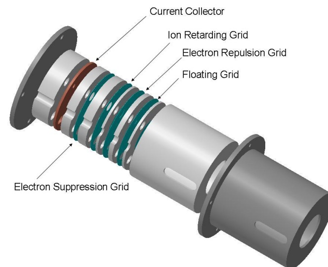
RPA (exploded view)
