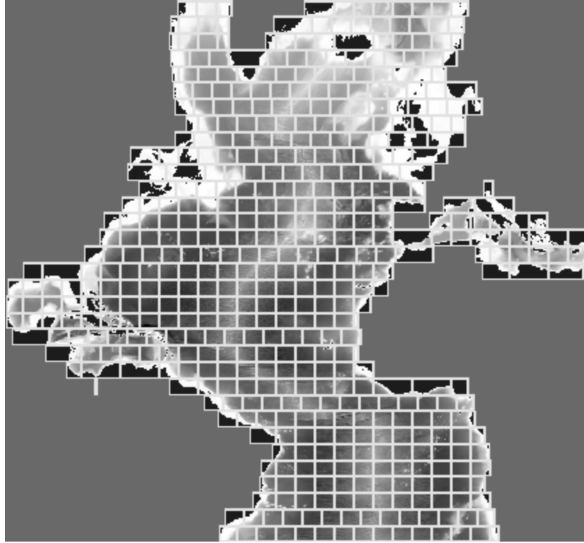
Figure 1: HYCOM 1/25^\circ Atlantic model domain decomposition for 507 MPI tasks
