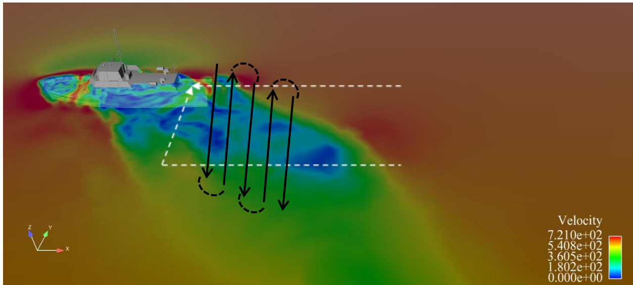
Figure 15. YP Air Wake for a 60° crosswind off the starboard bow. Black arrows represent a sample RC Helicopter flight profile to detect variation in ship air wake. White arrows represent common fleet helicopter approach paths.
