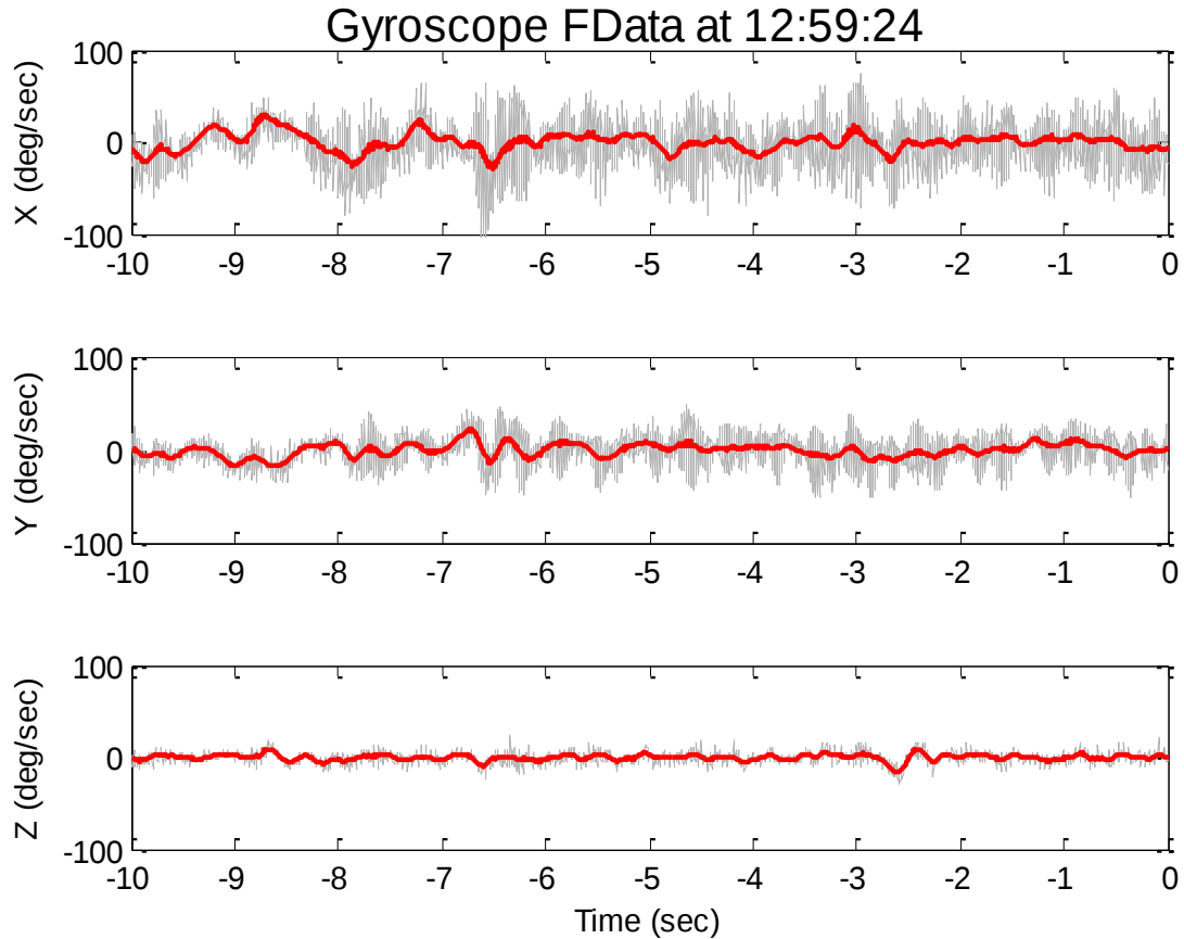
Figure 19. Filtered gyrosopic data plot.
