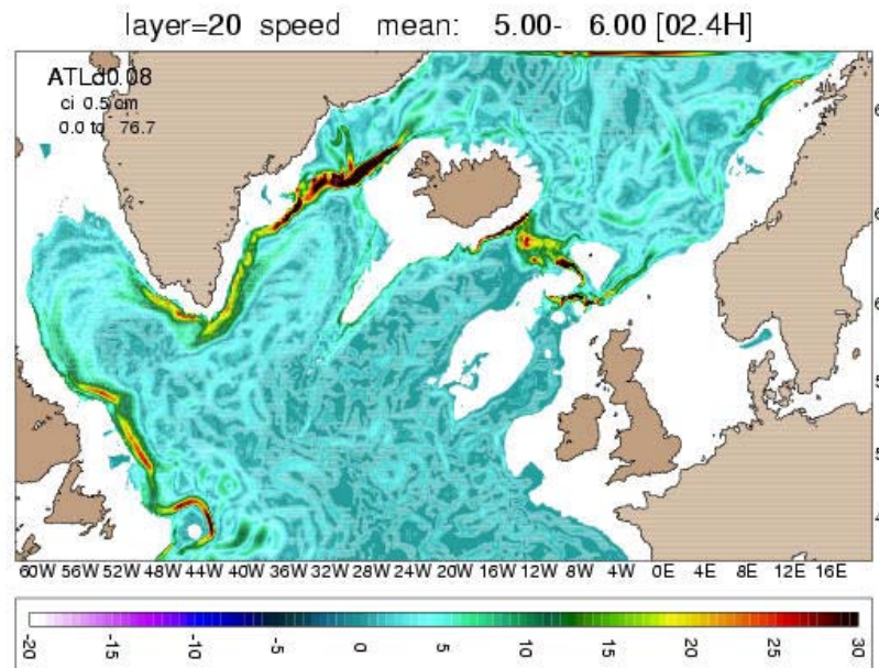
Figure 13. Proposed transport scheme for waters denser than \sigma_\theta = 27.80 in the northern North Atlantic, based on all available measurements.
