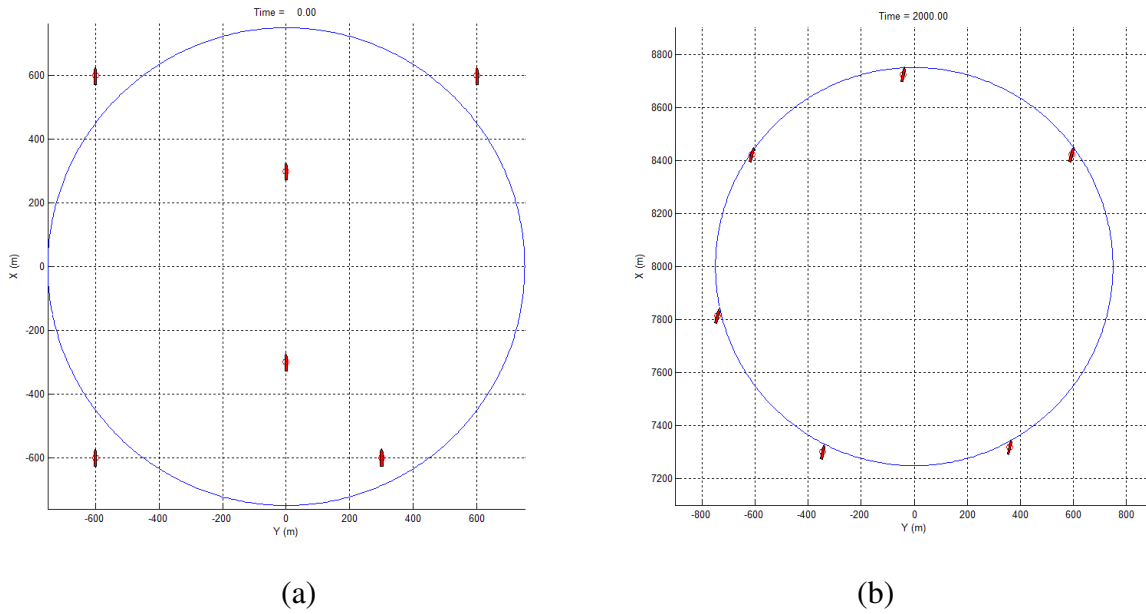
Figure 47 (a) Start and (b) End of Simulation with Circular Formation and no Curvature Optimization
