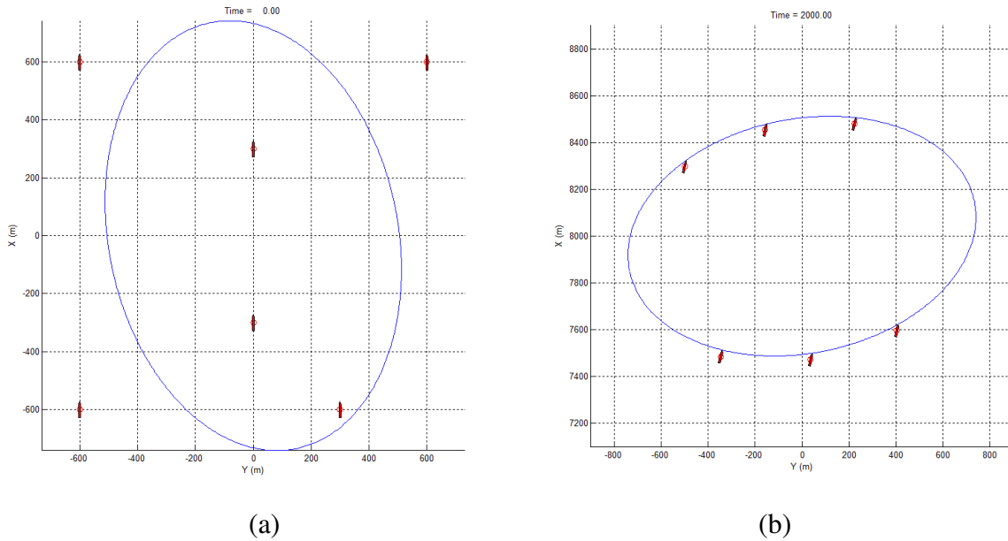
Figure 48: (a) Start and (b) End of Simulation with Method 1 of Curvature Optimization and Complimentary Elliptical Formation
