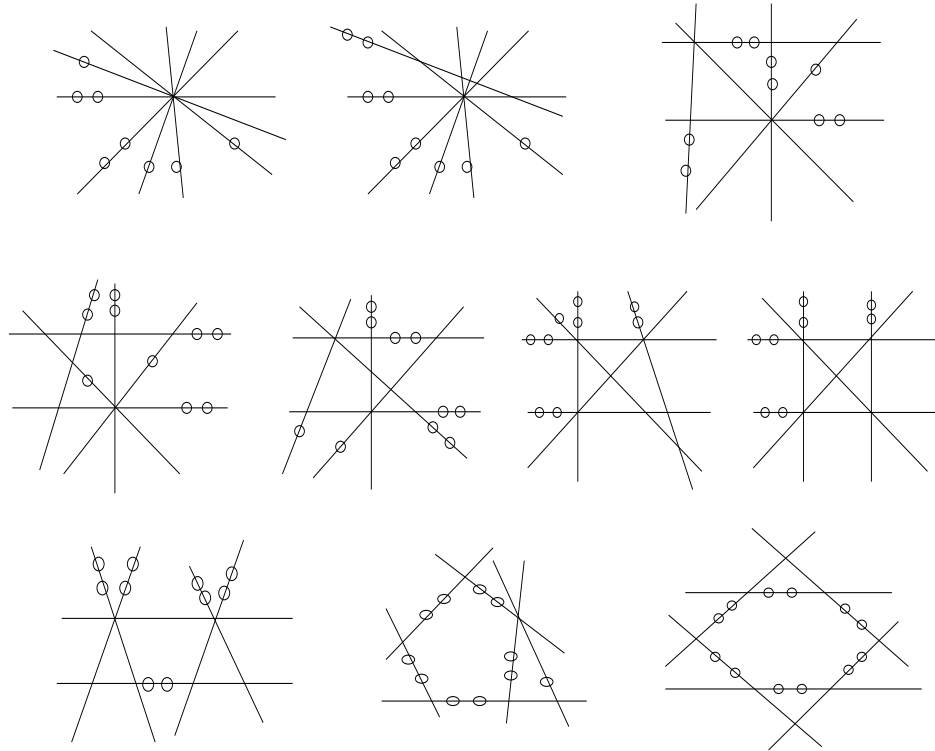
Figure 4: 10 Intersection Lattice Types for \ell = 6 lines
